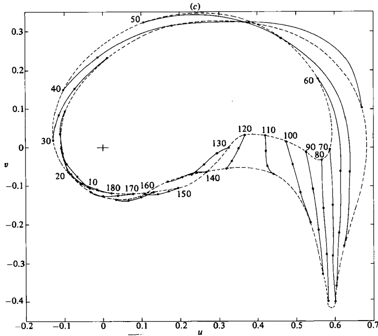
FIGURE 8. Velocity-plane portraits for the high-resolution computations of waves 1 (a), 3 (b) and 9 (c) (times as given in the text): —, particle trajectories; -----, envelopes of the starting and finishing positions. Particle numbers are indicated at the beginning of each trajectory.
