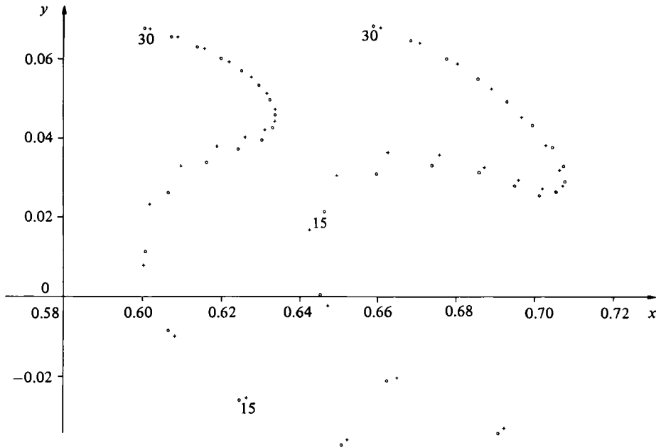
FIGURE 2. Comparison of the present method ( \circ ) with that of Vinje & Brevig (1981, + ) for a breaking sine wave. The profiles are at times t = 1.10 and t = 1.25 .
