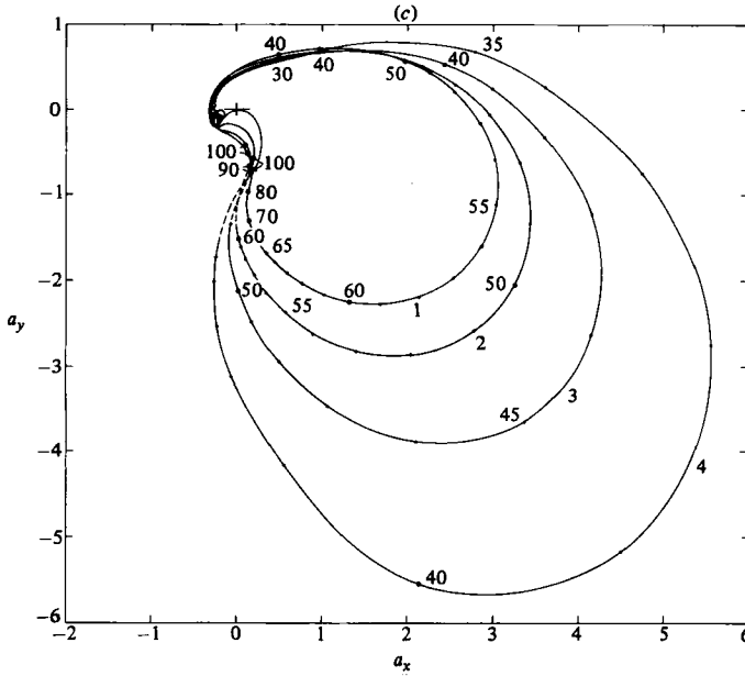
FIGURE 9. Acceleration-plane portraits for the high-resolution computations of waves 1 ( a ), 3 ( b ) and 9 ( c ): —, envelopes of the free-surface accelerations; -----, regions of unacceptable numerical error. The curves are numbered in the time sequence as given in the text, and the particles are marked as clarity allows ( \circ identifies every tenth and + every fifth).
