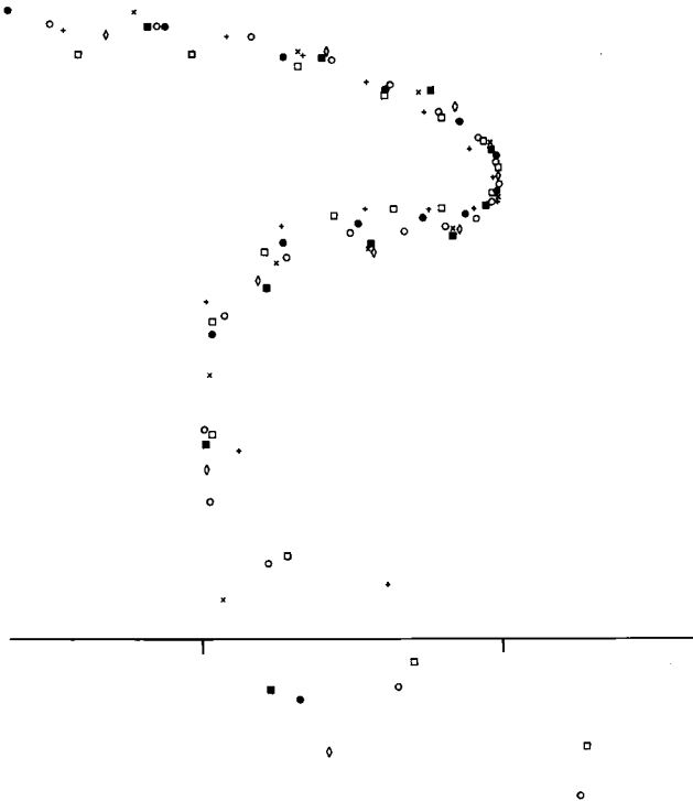
FIGURE 10. A selection of wave profiles shown at time t = t_H and scaled with respect to the jet length S (which is denoted by the tick marks on the arbitrary horizontal axis): \circ , wave 2; \bullet , 3; \square , 5; \blacksquare , 6; \diamond , 8; + , 9; \times , 10.
