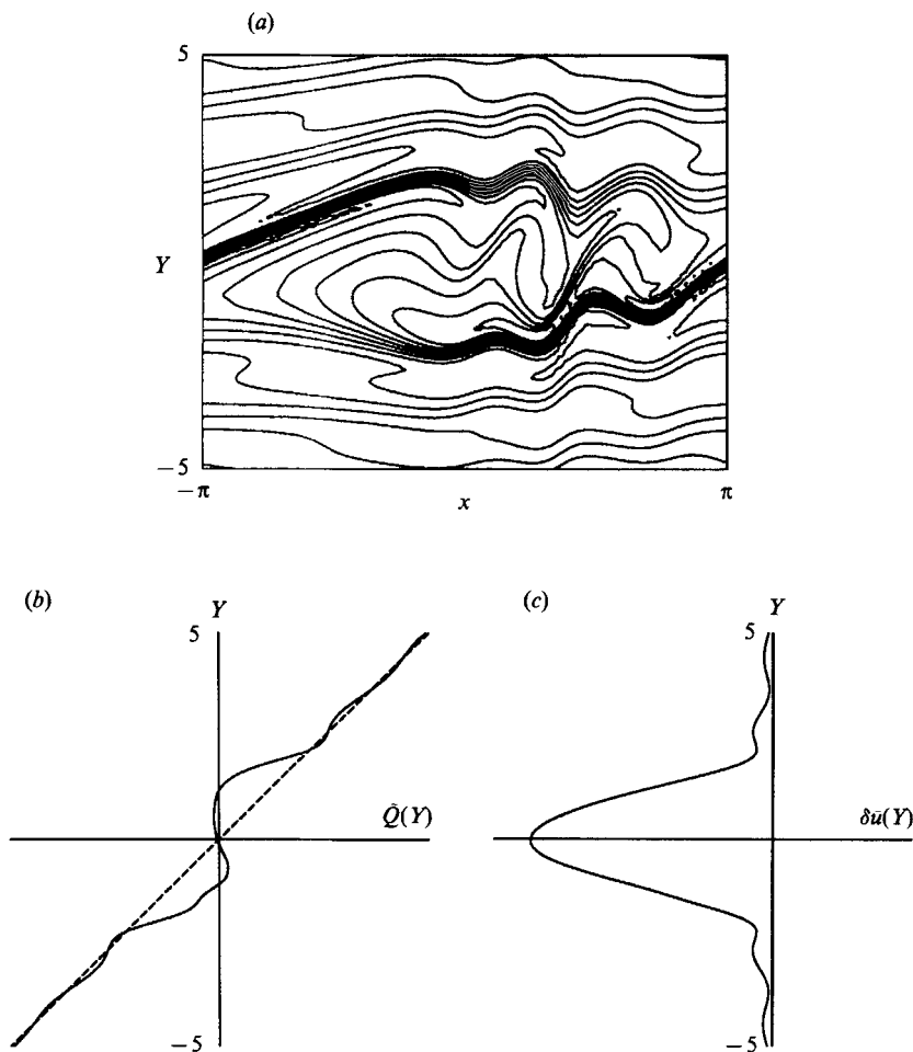
FIGURE 5. (a) Contours of Q or \zeta^2 in the narrow wave breaking or critical layer region in an inviscid, nonlinear Rossby-wave critical layer simulation like those described in Haynes (1989), except at higher numerical resolution. A combination of analytical and numerical techniques is used (both here and in the reference cited) in order to achieve this resolution. The width of the critical layer region is exaggerated for clarity. The contours in the central region of moderate values of Y , the stretched y or northward coordinate, are being irreversibly deformed to an extent that leads to a substantial irreversible rearrangement of Q and hence a substantial change in the eastward mean flow \bar{u}(Y) . (b) Eulerian-mean initial (dashed) and present (solid) \bar{Q}(Y) profiles, differing by \delta\bar{Q}(Y) say. (c) Eulerian-mean flow change \delta\bar{u}(Y) that results from the rearrangement. In this simple model the inversion operator that gives \delta\bar{u} in terms of \delta\bar{Q} is simply minus the y -integral of \delta\bar{Q} .
