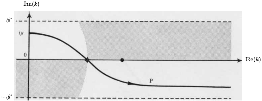
FIGURE 2. Path of integration, P , for (3.37 b ), when k_{0n} < k_n , i.e. when x < v_n t , upstream of the tail. The dot indicates the pole at k = k_n ; the path crosses the real axis at the saddle point k = k_{0n} .
