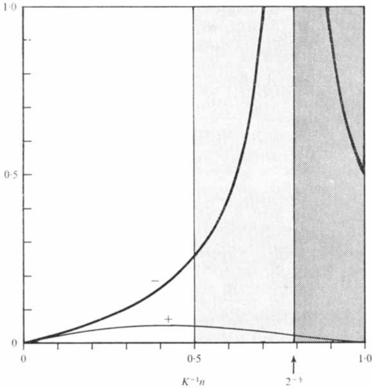
FIGURE 4. Strengths of the pair of columnar disturbances due to the n th lee-wave tail, as a function of K^{-1}n . Upon multiplying the ordinate by \mathbf{k}_n^2 |\mathbf{a}_n|^2 , the heavy curve gives \Gamma_{2n}^- , and the light curve gives \Gamma_{2n}^+ . (See text.)
