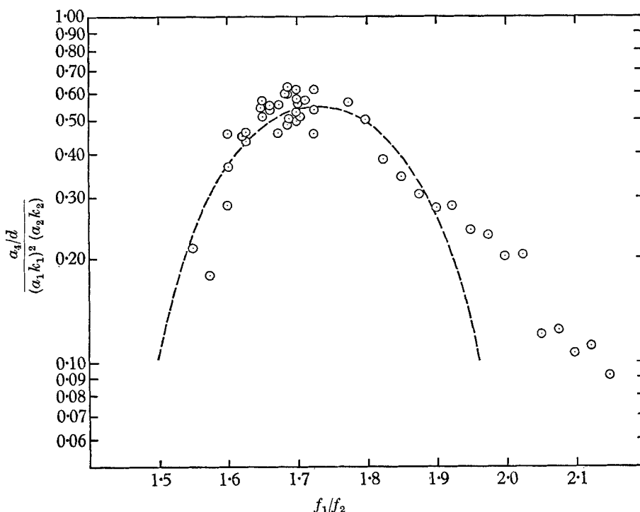
FIGURE 3. The resonant response at d = 81.4 cm, series I.
