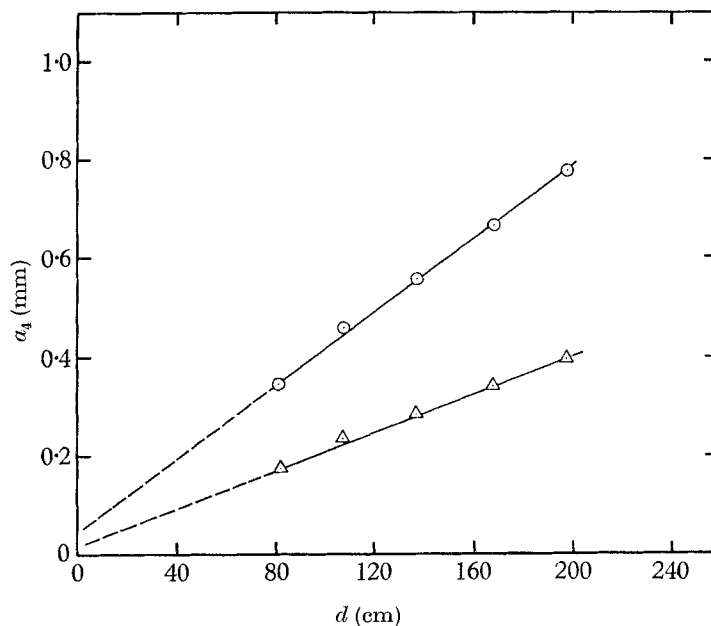
FIGURE 8. The measured growth of a_4 . \odot , Series I; \triangle , series II.
