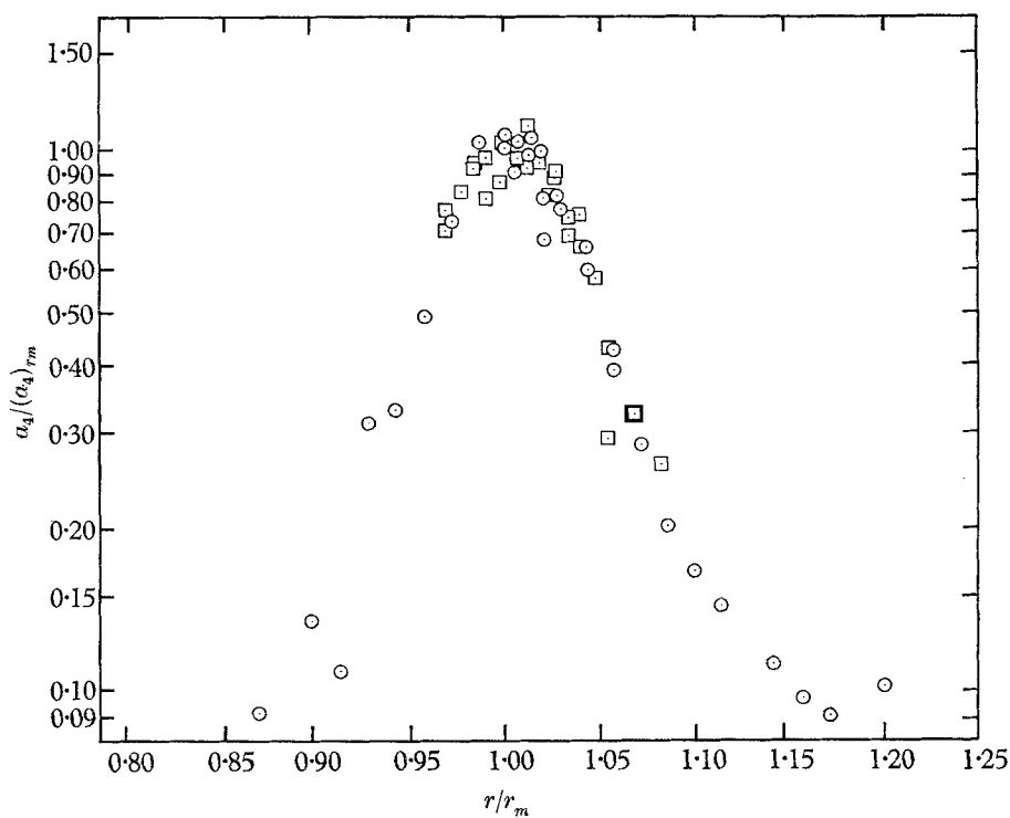
FIGURE 9. Comparison between resonant responses for series I and III. For series III, r_m = 1.775 . \odot , Series I; \square , series III; d = 198 cm.
