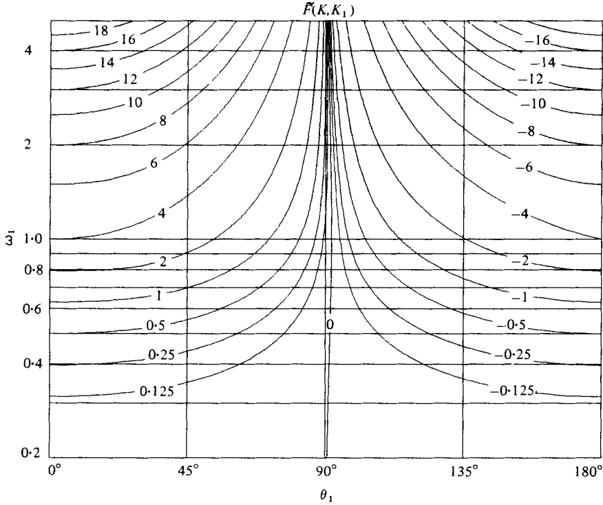
FIGURE 1. Contours of the kernel \tilde{F}(K, K_1) , where K = (\omega, \mathbf{k}) = \{\omega, |\mathbf{k}|, \theta\} is assigned as \{1, 1, 0\} while K_1 = \{\omega_1, |\mathbf{k}_1|, \theta_1\} is varied. The free wave K_1 is represented by two quantities, i.e. the frequency \omega_1 and the direction \theta_1 of propagation, because |\mathbf{k}_1| is determined from the dispersion relation.
