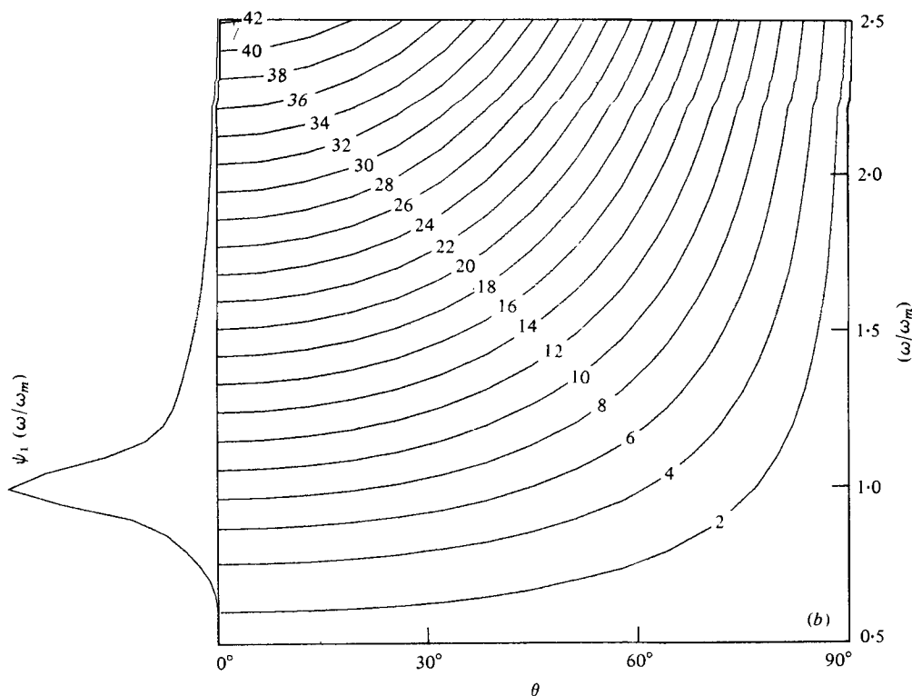
FIGURE 3. Contours as in figure 2 but for JONSWAP spectra. (a) A \cos^2\theta type directional distribution is assumed. (b) A \cos^8\theta type directional distribution is assumed.
