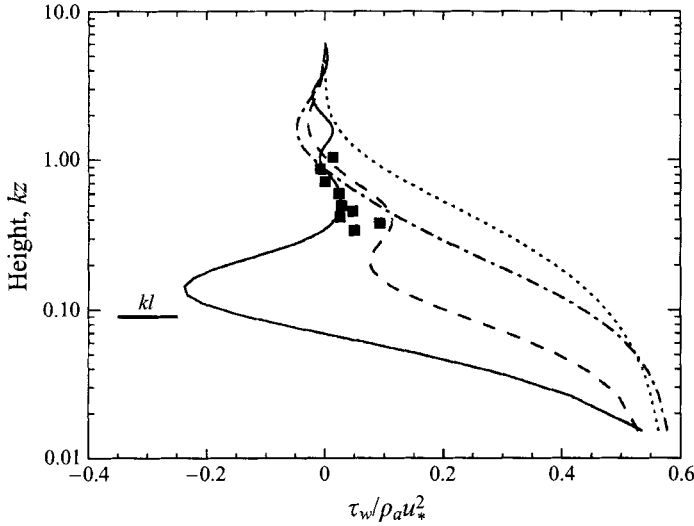
FIGURE 11. The mean wave stress as a function of height kz . According to the mixing length model (dash-dotted line) the wave stress decays slightly faster than \exp(-2kz) (dotted line). In the LRR scheme (solid line) the wave stress decays to zero at the top of the inner region, and shows an overshoot with reversed sign at the bottom of the outer region. The wave stress calculated with the e - e scheme is indicated with the dashed line. The solid squares indicate observed wave stresses in run BA.
