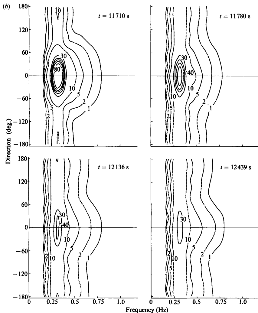
FIGURE 17. Time evolution of the spectrum, F(f, \theta) ( 10^{-3} \text{ m}^{-2} \text{ s rad}^{-1} ), in the presence of a partial ice cover of (a) 10 % and (b) 20 % with ice floes of radius a = 10 \text{ m} and draft d = 2 \text{ m} , U_{10} = 10 \text{ m/s} and f_{\text{peak}}(t_0) = 0.3 \text{ Hz} .
