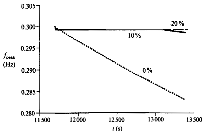
FIGURE 21. Time evolution of the peak frequency, f_{peak} , of an initial JONSWAP spectrum ( f_{peak} = 0.3 Hz) in the presence of a partial ice cover of 0% (from the Hasselmann parametric model), 10% and 20%.
