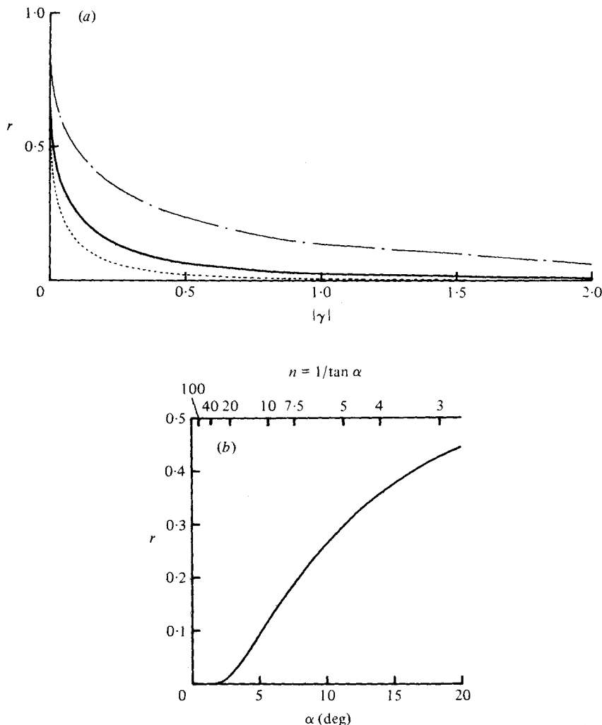
FIGURE 3. (a) The reflexion coefficient r as a function of the parameter |\gamma| , according to (4.12). —, r_0 ; — · —, r_{|\gamma|} ; · · · · ·, r_{-|\gamma|} . (b) The dependence of r_0 on the beach slope for \omega = 9.06 \text{ s}^{-1} , \nu = 0.01 \text{ cm}^2 \text{ s}^{-1} .
