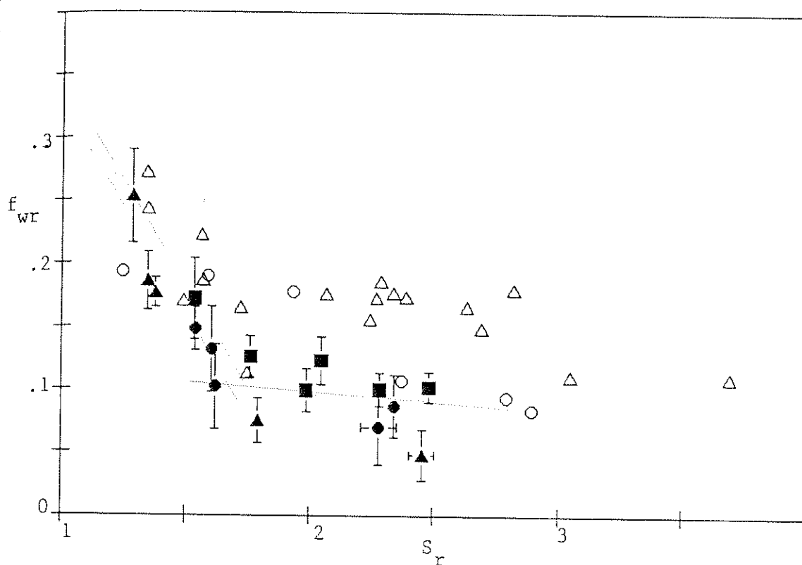
Figure 1. Movable bed friction factors for spectral waves (solid symbols) and periodic waves (open symbols). Triangles: 0.2-mm, Pierson-Neumann spectrum; circles: 0.12-mm, Pierson-Neumann spectrum; squares: 0.12-mm, finite-depth Jonswap spectrum
