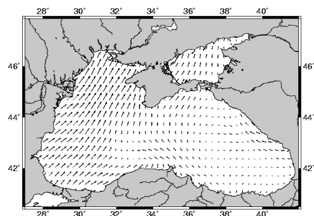
Figure 1 Wind field at 10 m predicted by MM5 at 10.00 UTC 25 September 2002
