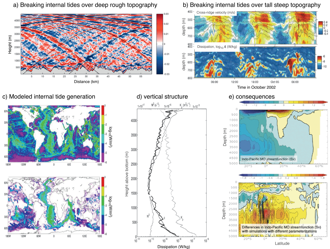
FIG. 3. (a) A snapshot of baroclinic velocity ( \text{m s}^{-1} ) from a two-dimensional numerical simulation of internal tides forced by M_2 (semidiurnal) tidal velocities over rough topography for parameters corresponding to the Brazil Basin (Nikurashin and Legg 2011). (b) Observational time series of internal wave breaking over tall steep topography; here, we see (top) northward velocity and (bottom) turbulent dissipation rate oscillate twice a day as the tide flows over Kaena Ridge, Hawaii (Klymak et al. 2008). (c) Global energy flux from the M_2 tide into internal tides ( \log_{10} W \text{ m}^{-2} ) estimated using (top) the topography resolved in the Shuttle Radar Topography Mission (SRTM) global bathymetry and elevation data at 30 arc s resolution with data voids filled (SRTM30 PLUS) bathymetry database and (bottom) a statistical representation of unresolved abyssal hill topography estimates (Melet et al. 2013b). (d) The vertical structure of dissipation from Brazil Basin observations (thick solid curve) and the Polzin (2009) [Eq. (4)] parameterization of near-field internal tide dissipation (thin solid curve), as well as associated observed values of stratification ( N^2 ) and diapycnal diffusivity ( K_p ). (e) The impact of the Polzin (2009) parameterization in the GFDL CM2G coupled climate model: (top) the Indo-Pacific meridional overturning streamfunction (Sv; 1 \text{ Sv} = 10^6 \text{ m}^3 \text{ s}^{-1} ; averaged over the final 100 years of a 1000-yr simulation) using the Polzin (2009) parameterization and (bottom) the differences in Indo-Pacific meridional overturning streamfunction (Sv) between the simulations with the Polzin (2009) parameterization and the St. Laurent et al. (2002) parameterization as implemented by Simmons et al. (2004b) (from Melet et al. 2013a).
