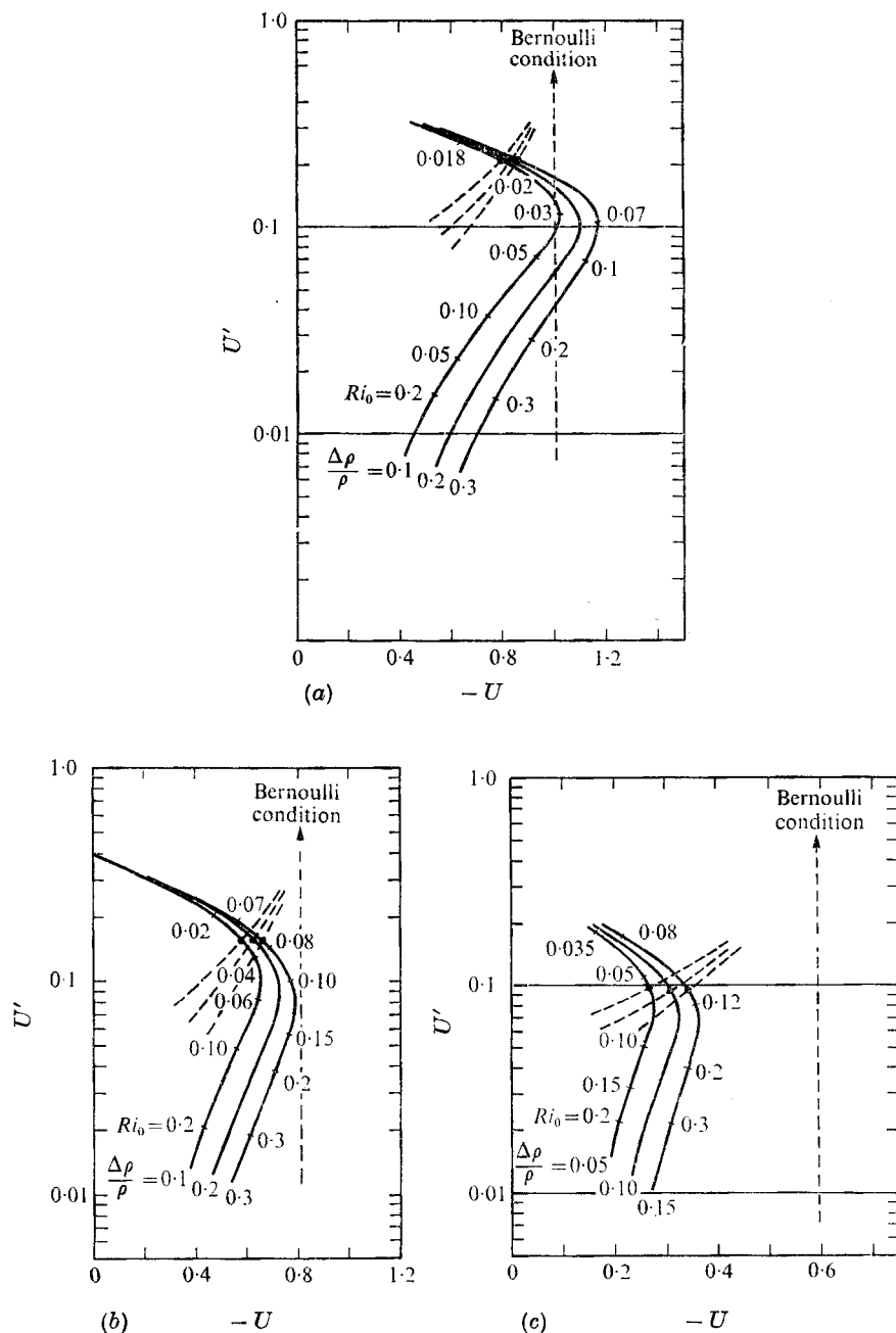
FIGURE 4. Non-dimensional whitecap velocity U' plotted against the upslope velocity U in the laminar flow below. (a) Slope of 30^\circ . (b) Slope of 20^\circ . (c) Slope of 10^\circ . Plots for three density differences are given in each case; values of Ri_0 are marked on the curves. The vertical dashed line is drawn at the value of U obtained using the Bernoulli relation, and the inclined dashed lines show the modification due to the pressure effect of the whitecap.
