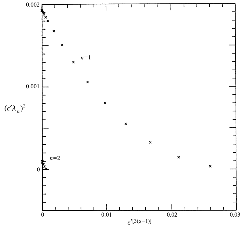
FIGURE 7. Scaled values of the squared growth rates of the two lowest modes of instability of the solitary wave, as a function of \epsilon'[3(\alpha-1)] .
