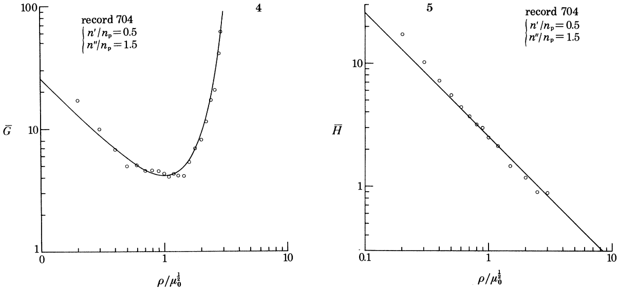
FIGURE 4. Plot of the mean group length \bar{G} corresponding to figure 1 d, as a function of the critical level. The theoretical curve represents (4.5). FIGURE 5. Plot of the mean length of high runs \bar{H} corresponding to the record of figure 1 d. The line represents (5.5).
