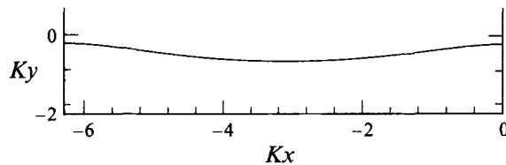
FIGURE 16. The theoretical profile for a wave with L = 10.2 cm, AK = 0.25 , by the method of §7.
