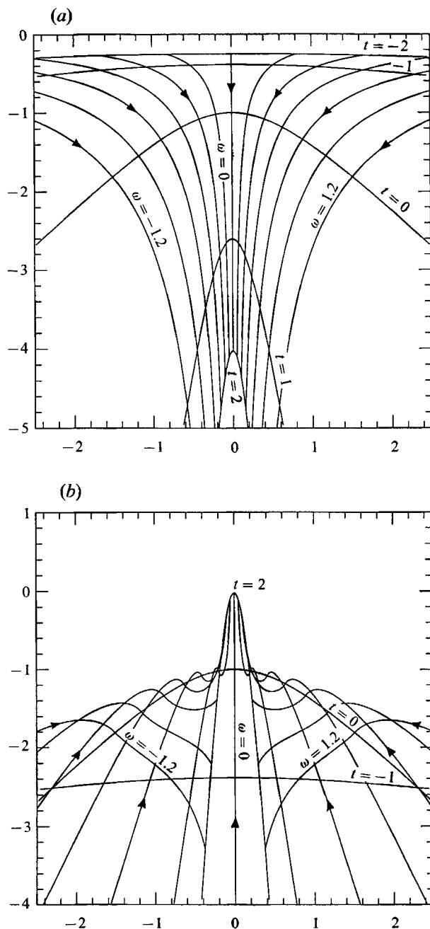
FIGURE 12. Particle paths in a Dirichlet hyperbola. (a) V = 0 ; (b) V = 2 .
