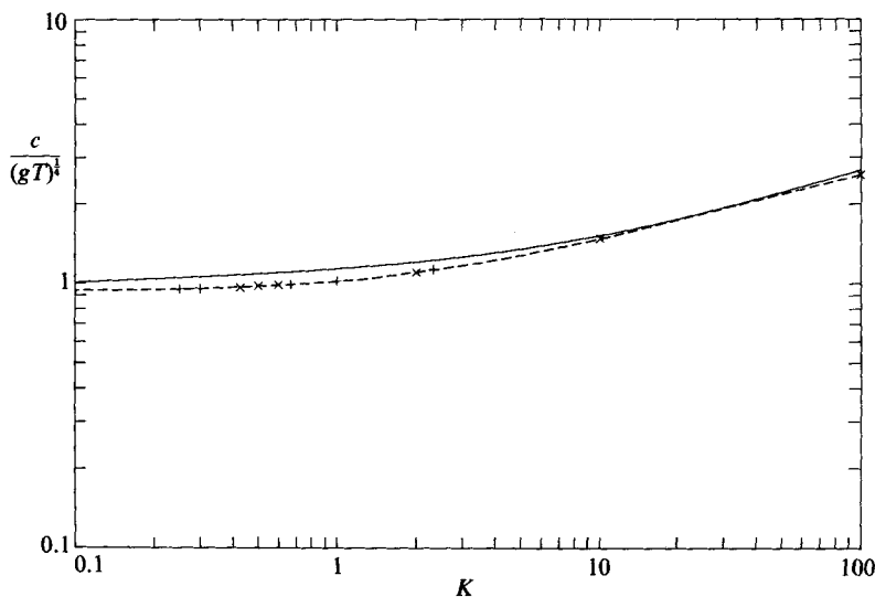
FIGURE 14. The dimensionless phase speed c/(gT)^{\frac{1}{4}} in a capillary-gravity wave of limiting steepness, as a function of K . Full curve represents the vortex approximation; plotted points fully calculated values: \times , Schwartz & Vanden-Broeck (1979); + , Chen & Saffman (1980).
