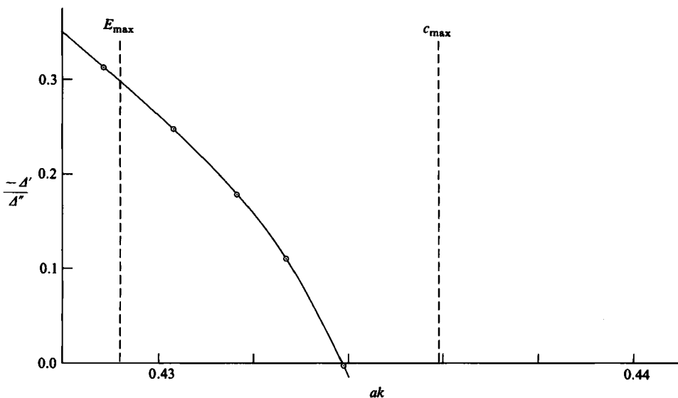
FIGURE 2. The ratio \Delta'/\Delta'' for the matrix of (5.5).
