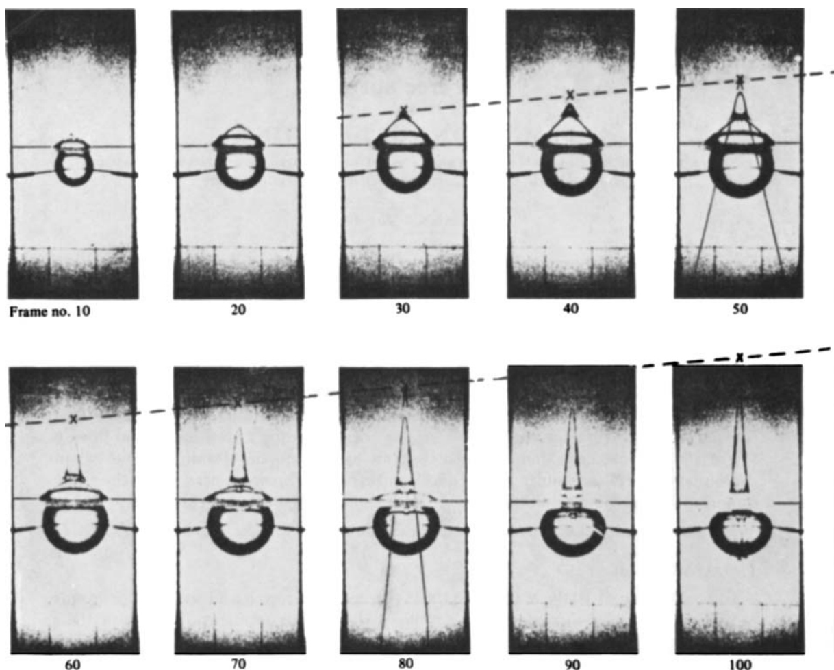
FIGURE 1. Jet produced by a gas bubble approaching a free surface (after Blake & Gibson 1981). The dashed line represents the trajectory of the assumed centre of the hyperboloid.
