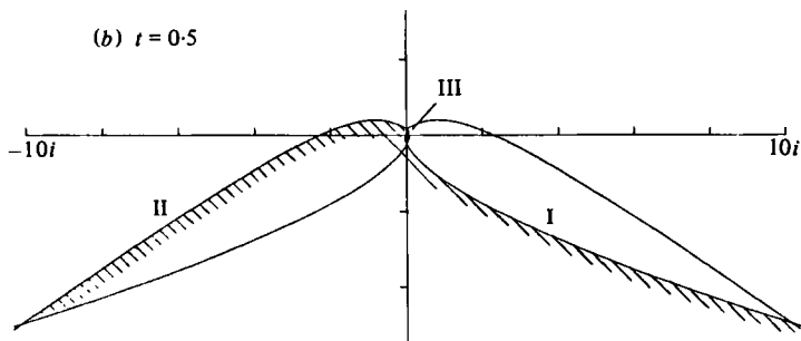
FIGURE 13. Contours of the pressure for z = P_3 in the physical plane: (a) when t = 1 ; (b) when t = 0.5 .
