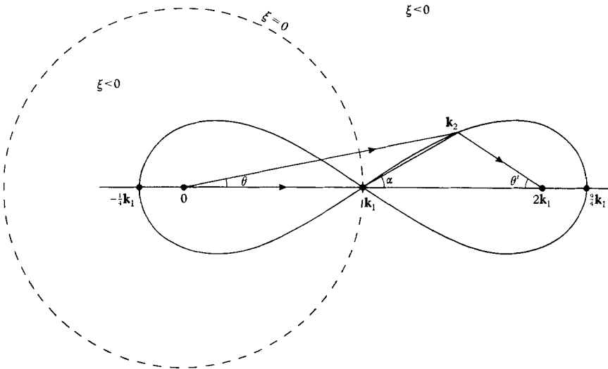
FIGURE 2. Locus of \mathbf{k}_2 , when \mathbf{k}_1 is fixed.
