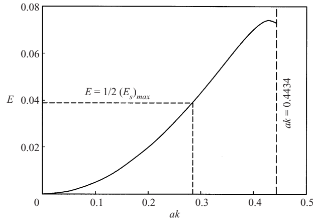
FIGURE 2. Graph of the energy density E_p of a progressive gravity wave of finite steepness ak .
