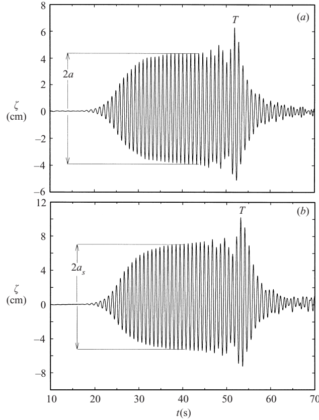
FIGURE 6. Surface elevation at x = 15.65 m when G = 1.6 (a) with no barrier and (b) with the barrier in place.
