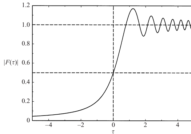
FIGURE 4. Theoretical envelope of the surface elevation in the neighbourhood of a wave front, from equation (4.1).
