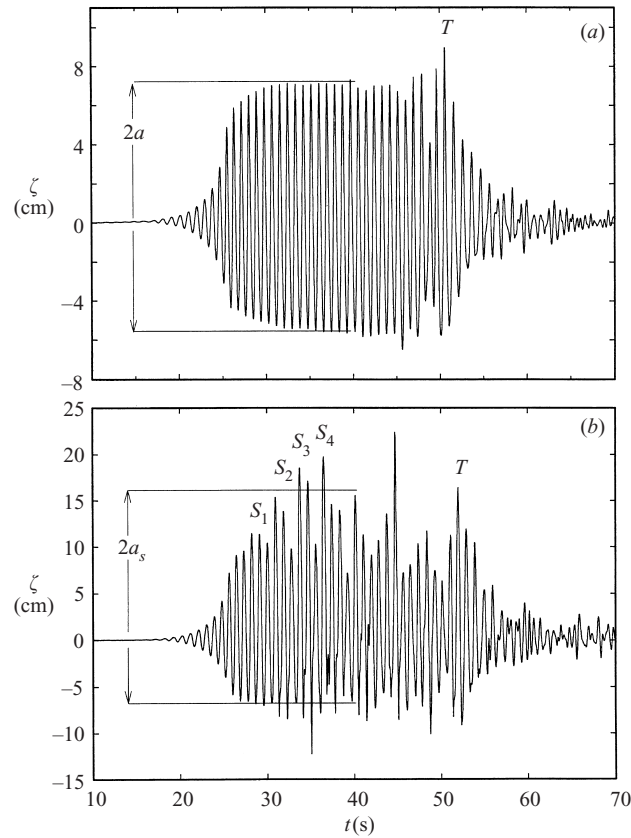
FIGURE 10. Surface elevation at x = 15.65 m when G = 2.6 (a) with no barrier (b) with the barrier in place.
