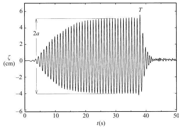
FIGURE 5. Record of the surface elevation at x = 2.30 m when \lambda = 0.1 and N = 40 (progressive wave: G = 1.6 ).
