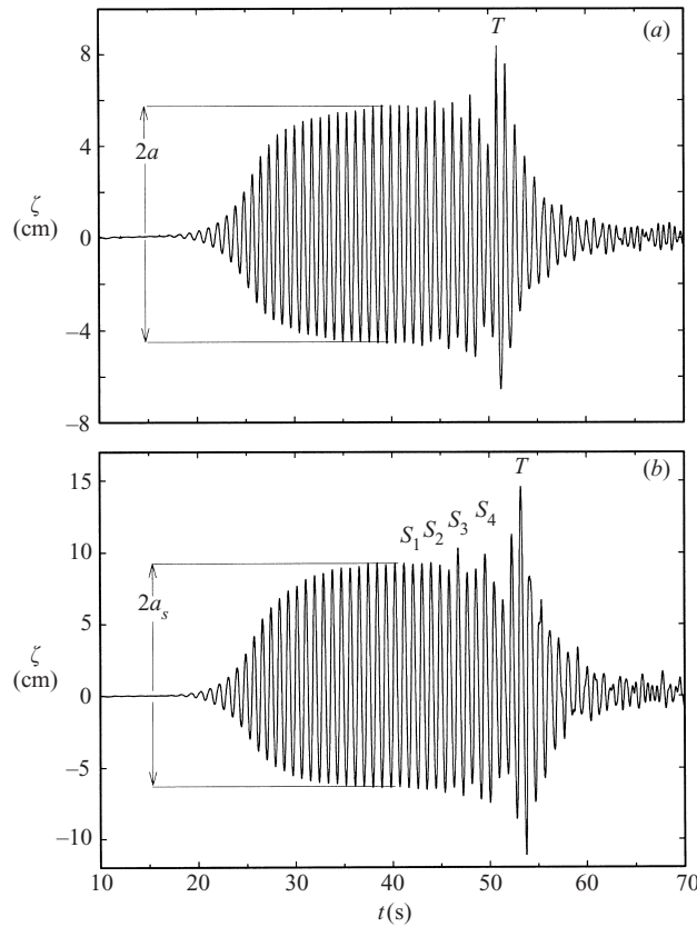
FIGURE 7. Surface elevation at x = 15.65 m when G = 2.0 (a) with no barrier (b) with the barrier in place.
