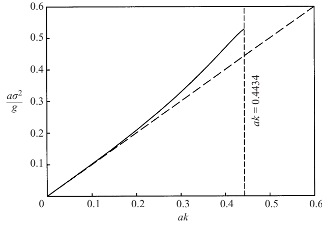
FIGURE 13. Graph of a\sigma^2/g against ak for nonlinear progressive gravity waves in deep water.
