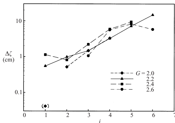
FIGURE 12. Growth of the triple-period instability, as measured by the difference \Delta\zeta in crest-elevation between the highest and lowest waves of a triplet.
