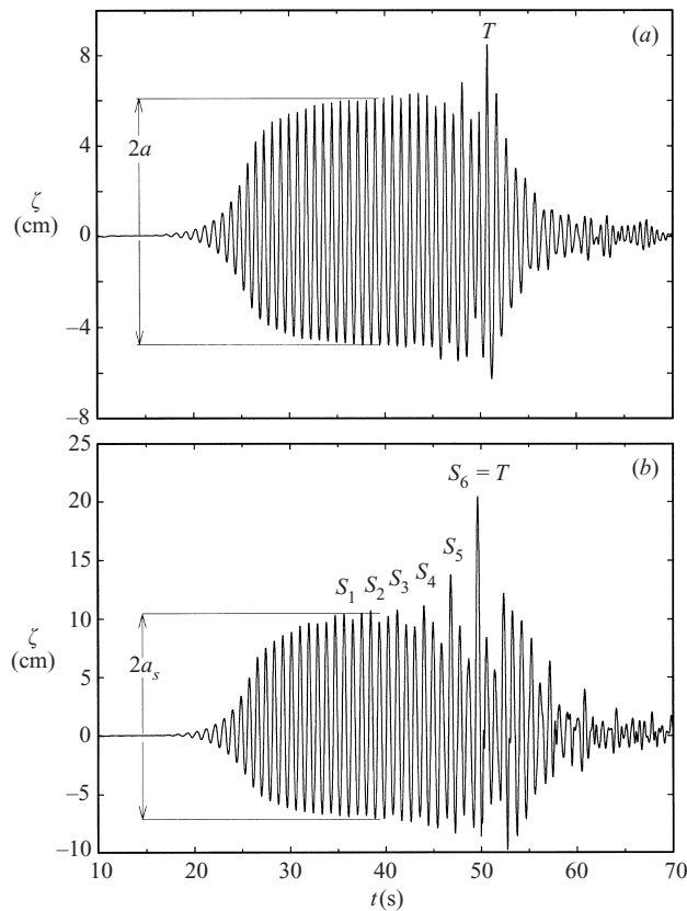
FIGURE 8. Surface elevation at x = 15.65 m when G = 2.2 (a) with no barrier (b) with the barrier in place.
