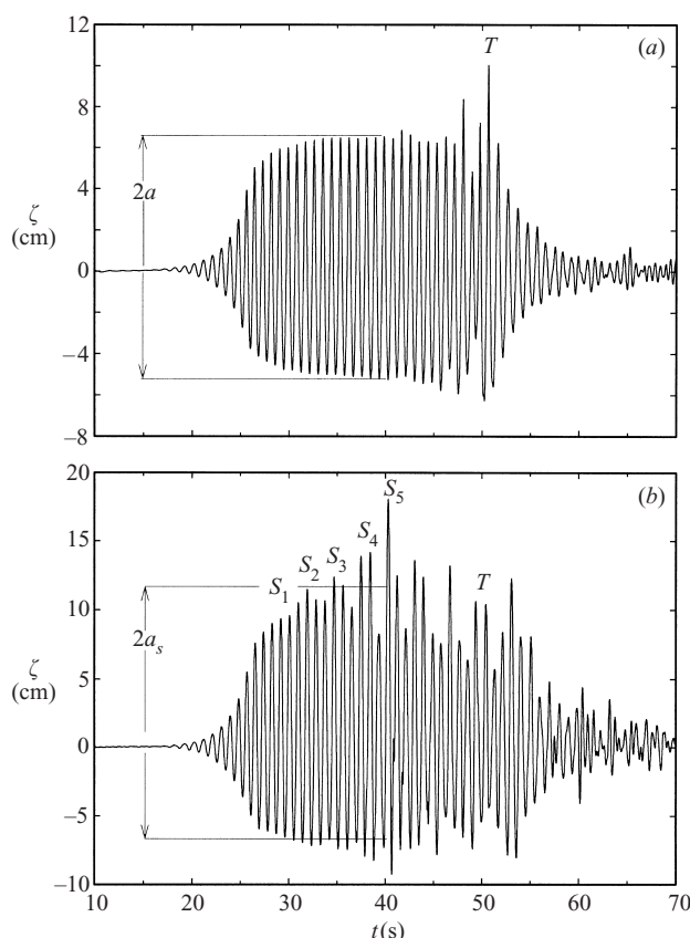
FIGURE 9. Surface elevation at x = 15.65 m when G = 2.4 (a) with no barrier (b) with the barrier in place.
