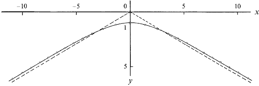
FIGURE 1. Profile of the almost-highest wave, showing coordinates and the 30^\circ asymptotes (from LHF1).
