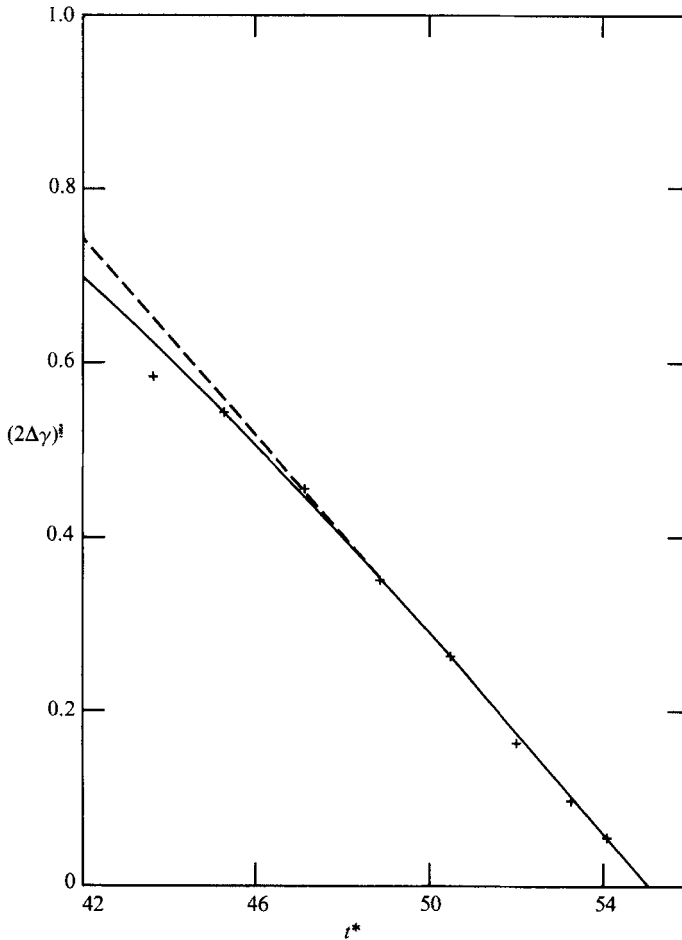
FIGURE 12. A plot of (2\Delta\gamma)^{1/2} versus the dimensionless time t^* corresponding to figure 11.
