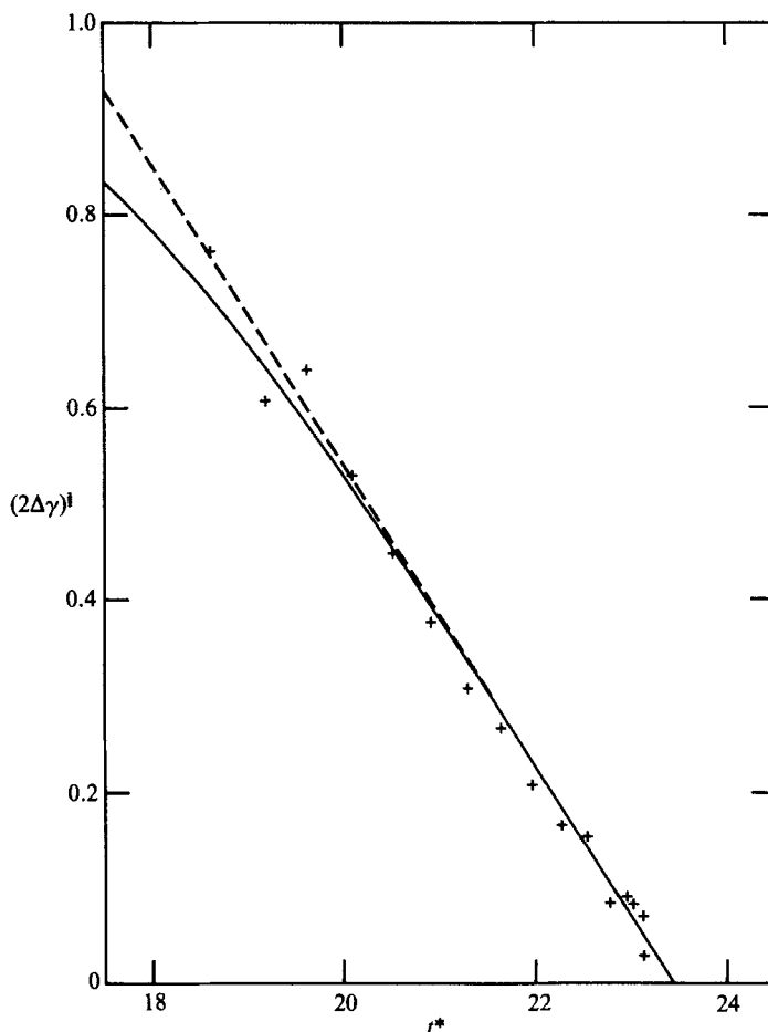
FIGURE 10. A plot of (2\Delta\gamma)^{\frac{1}{3}} versus the dimensionless time t^* corresponding to figure 3 (Oguz & Prosperetti 1989a). figure 11c), U = 1.75 m/s, R = 1 mm.
