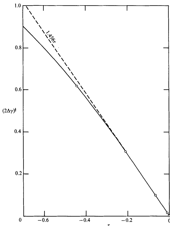
FIGURE 9. Graph showing the behaviour of the vertex angle 2\gamma in the neighbourhood of the critical instant t = 0 . Full curve represents (2\Delta\gamma)^{1/2} , from calculated values in table 1 of Longuet-Higgins (1983). Broken line represents linear asymptote.
