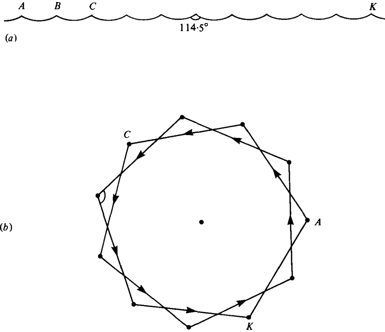
FIGURE 12. The transformation of 11 ripples with crest angle 114.50^\circ into the polygon \{11/2\} , (a) in the z plane and (b) in the \zeta plane.
