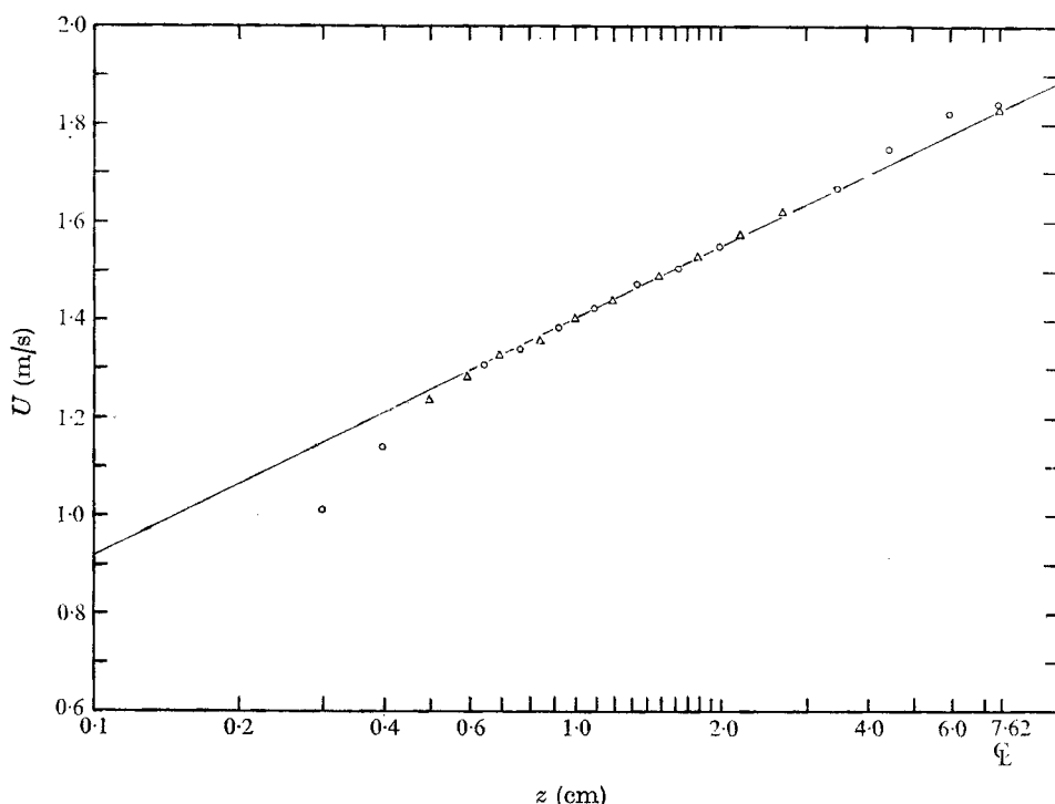
FIGURE 4. Axial component U of mean wind velocity for centre-line wind velocity of 1.84 \text{ m/s} expressed as a function of height z above mean water level. \Delta , 3 August 1971; \circ , 5 August 1971. Slope of line corresponds to U_* = 8.4 \text{ cm/s} , \kappa = 0.4 . All measurements made with 3.54 \text{ Hz} waves on water surface.
