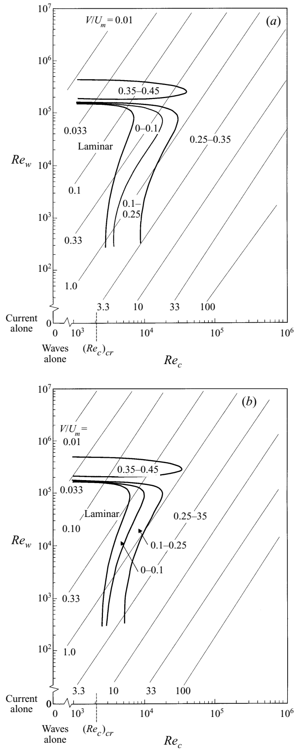
FIGURE 9. Contour plot of ((\tau_0^2)_{max})^{1/2} / \tau_{max} (see figure 8 for the definition): (a) R/\delta = 53 , (b) R/\delta = 25 .
