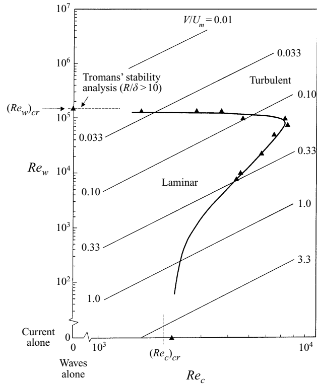
FIGURE 5. Transition to turbulence in combined flow. R/\delta = 53 .
