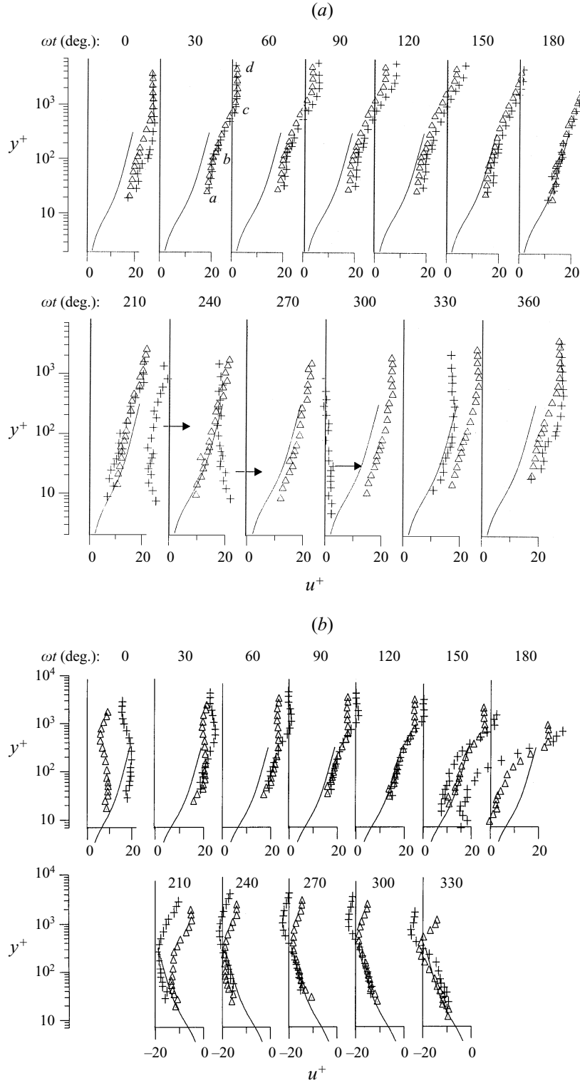
FIGURE 21. (a) Profiles of the ensemble-average velocity at different phase values. Combined flow. R/\delta = 53 . Re_c = 1.6 \times 10^5 . Triangles: Re_w = 0.7 \times 10^6 , V/U_m = 1.3 . Crosses: Re_w = 2.4 \times 10^6 , V/U_m = 0.7 . Solid lines: van Driest profile (equation (18)). (b) As (a) but Re_c = 2.7 \times 10^4 . Triangles: Re_w = 0.7 \times 10^6 , V/U_m = 0.2 . Crosses: Re_w = 2.4 \times 10^6 , V/U_m = 0.1 .
