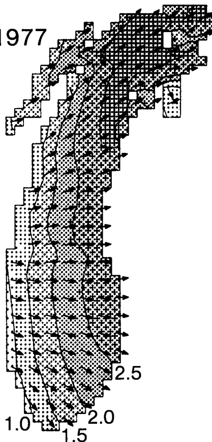
FIG. 6. As in Fig. 5 except for west wind, 21 November 1977.
