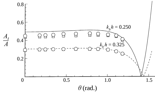
FIGURE 15. Class III Bragg super-harmonic transmission coefficient as a function of incidence wave angle \theta relative to the bottom ripples, for kA = 0.03 , k_b d = 0.025 and L_0/\lambda_b = 5 . Results plotted are: regular perturbation solutions (—) for k_b h = 0.25 and (---) for k_b h = 0.325 ; and HOS computations for M = 3 ( \square ) and M = 4 ( \circ ) for the respective mean depths.
