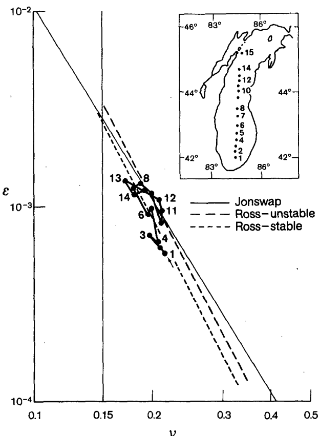
FIG. 8. As in Fig. 7 except for 2019–2106 on 20 November.
