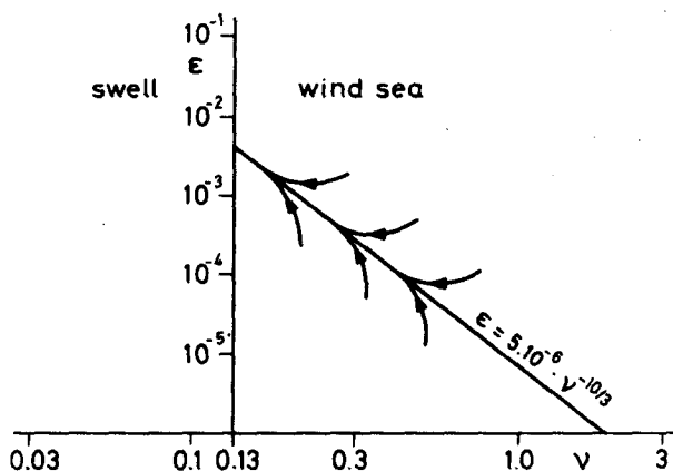
FIG. 6. Wave growth in the \epsilon vs \nu plane (after Hasselmann et al., 1976).
