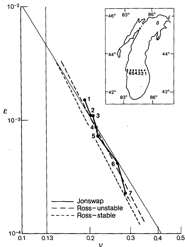
FIG. 10. As in Fig. 7 except for 1916–1932 on 21 November.
