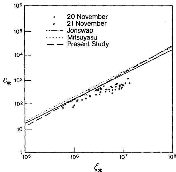
FIG. 13. Correlating \epsilon_* vs \xi_* for wave growth data on 20 and 21 November.
