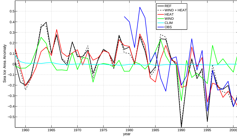
FIG. 5.2: Annual anomaly of the Arctic sea ice area ( 10^6 \text{ km}^2 ) for the different simulations. Satellite observations are also shown for comparison ( Fetterer et al. , 2002, updated 2009).
