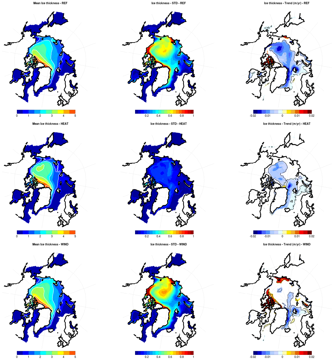
FIG. 5.6: Average over 1963–2001, standard deviations and linear trends of the sea ice thickness for the REF (top), HEAT (middle) and WIND (bottom) experiments. Only trends that reach a 90% significance level are shown and the black dotted line indicates the 95% significance level.
