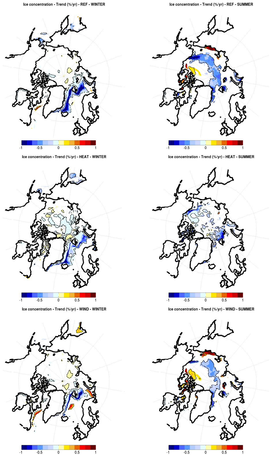
FIG. 5.3: Linear trends over 1963–2001 of the winter (left) and summer (right) mean sea ice concentration for the REF (top), HEAT (middle) and WIND (bottom) experiments. Only trends that reach a 90% significance level are shown and the black dotted line indicates the 95% significance level.
