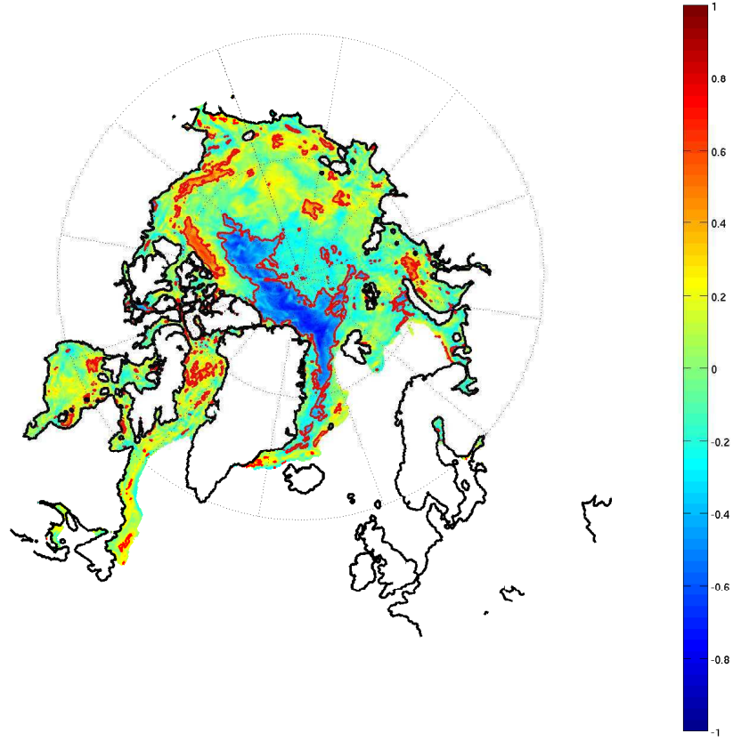
FIG. 2.14: Correlation between the ocean freshwater flux through Fram Strait and the ocean-ice flux over the Arctic domain. Calculations are done over the 1965–2002 period for the EXP1 run. The 95% significance level is indicated in red (based upon 36 degrees of freedom, which is an upper limit).
