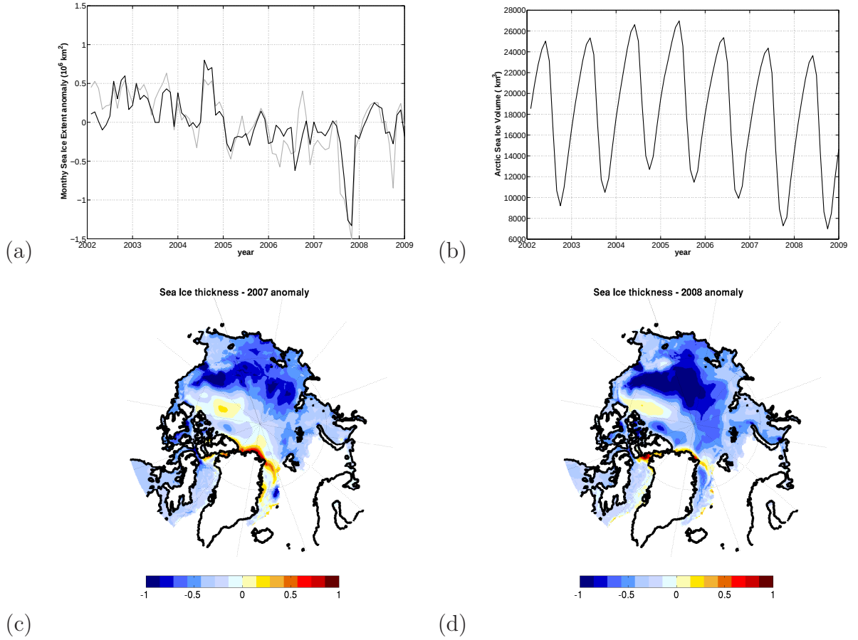
FIG. 3.1: GLORYS1 monthly Arctic Sea Ice Extent anomaly (a) and Volume (b). NSIDC observed Sea Ice Extent is superimposed in gray for direct comparison (Fetterer et al. , 2002, updated 2009). The sea ice volume can be compared to Kwok et al. (2009) (Fig.5). Sea ice thickness anomalies (meters) in 2007 (c) and 2008 (d). "Anomaly" refers to the difference with the average over 2002–2006.
