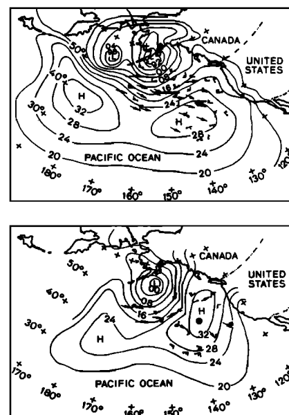
Fig. 2. National Weather Service surface charts compiled for May 17, 1978 (top) 0000 UT, (bottom) 1800 UT. The location of the NOAA Data Buoy 46006 is indicated by the solid circle.
