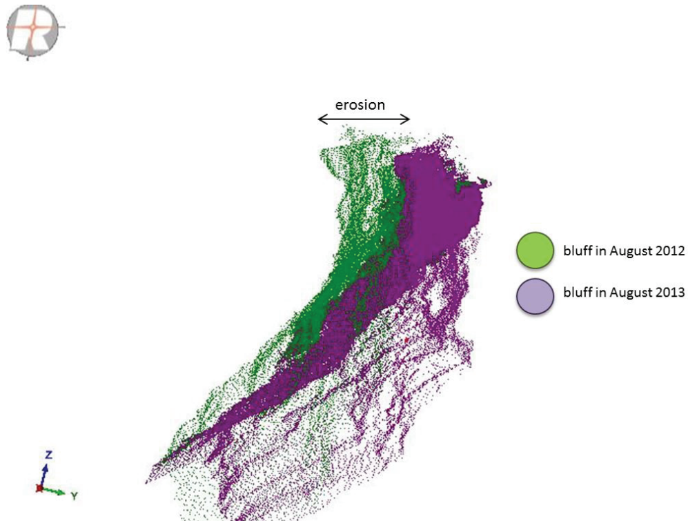
Figure 5: Profile of the scanned coastal bluff (pointcloud section 3, 16m length), comparison of the recorded pointclouds of 2012 and 2013.
