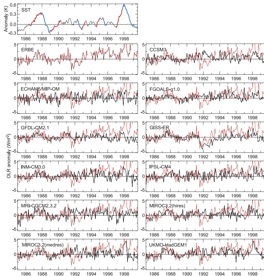
Figure 1a. Monthly SST, and TOA OLR from ERBE (red) and AMIP models (black) for 20°S–20°N. The major SST intervals for which \Delta\text{SST} exceeds 0.2°C are indicated by red and blue colors.
