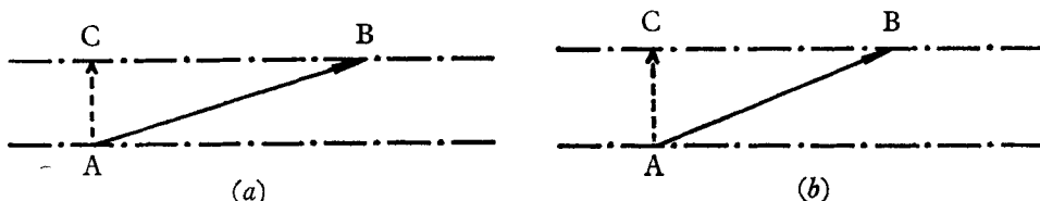
FIGURE 1. Flow viewed from downstream (a) at time t , (b) at time t + \delta t . - - - - , Pair of nearby horizontal lines of fluid perpendicular to the flow; A \rightarrow B arrow-shaped element in direction of vorticity, with length proportional to its magnitude; A \rightarrow C vertical resultant of element AB , with length proportional to vertical component of vorticity.
