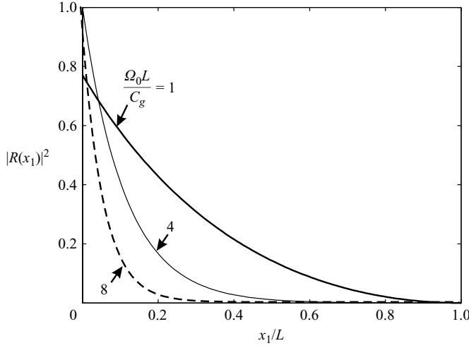
FIGURE 5. Reflection intensity along the array for various \Omega_0 L / C_g with detuning parameter \Omega / \Omega_0 = 0.5 . Thick solid curve: \Omega_0 L / C_g = 1 , thin solid curve: \Omega_0 L / C_g = 4 , dashed curve: \Omega_0 L / C_g = 8 .
