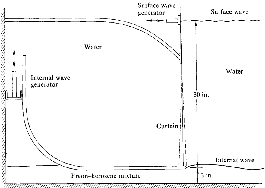
FIGURE 2. Schematic diagram of wave generators.
