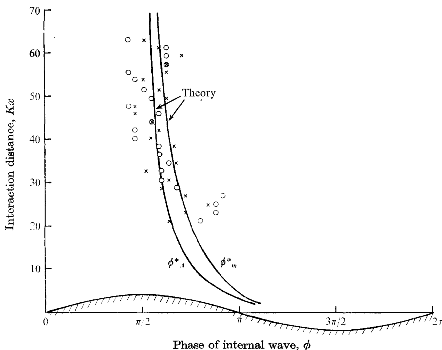
FIGURE 11. Effect of interaction 'distance' Kx on phase of internal wave where maximum slope and amplitude modulations occur for 'resonant' interactions. C/C_0 \approx 1 . \circ , \phi^* at m_{\max}^* ; \times , \phi^* at A_{\max}^* .
