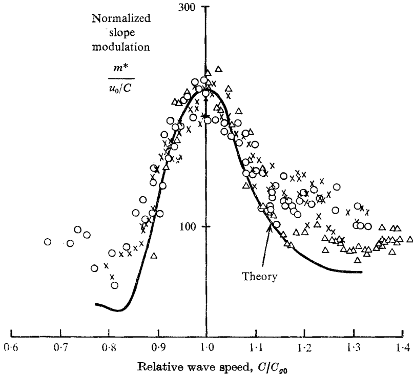
FIGURE 14. Normalized slope modulation against relative wave speed. Kx \simeq 43 .
