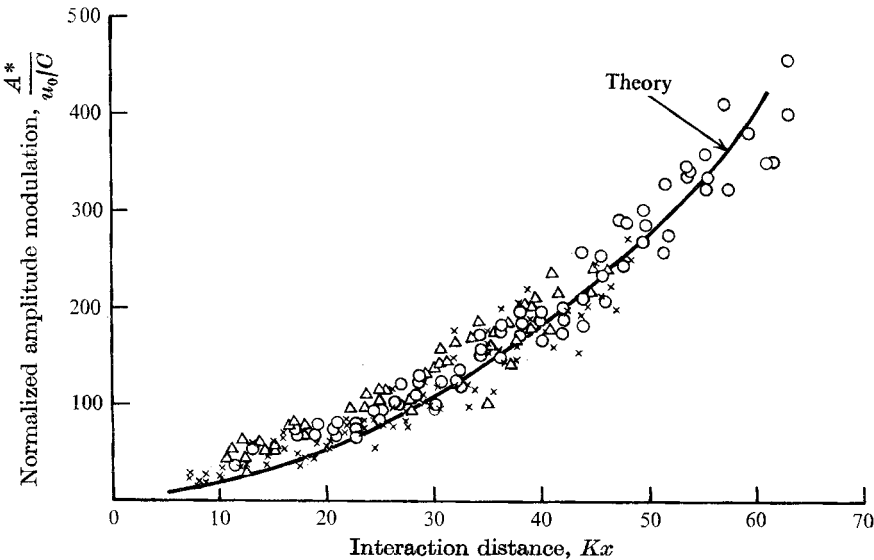
FIGURE 13. Normalized amplitude modulation against interaction ‘distance’ Kx . C/C_{g0} \simeq 1 . Symbols as in figure 12.
