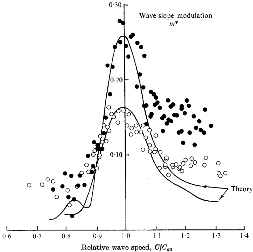
FIGURE 7. Surface-wave slope modulation against relative wave speed, equivalent interaction configurations at two values of Kx .
