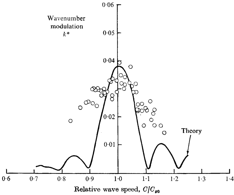
FIGURE 9. Surface-wavenumber modulation against relative wave speed for Kx = 58 , \rho = 1.152 , T_i = 3.9 s, K = 1.93 ft ^{-1} , x = 30 ft, u_0 = 5.54 \times 10^{-4} ft s ^{-1} .
