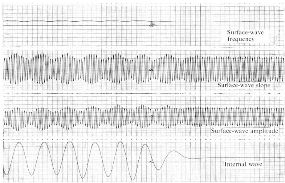
FIGURE 4. Oscillograph records, showing onset of interaction of internal wave with surface wave.
