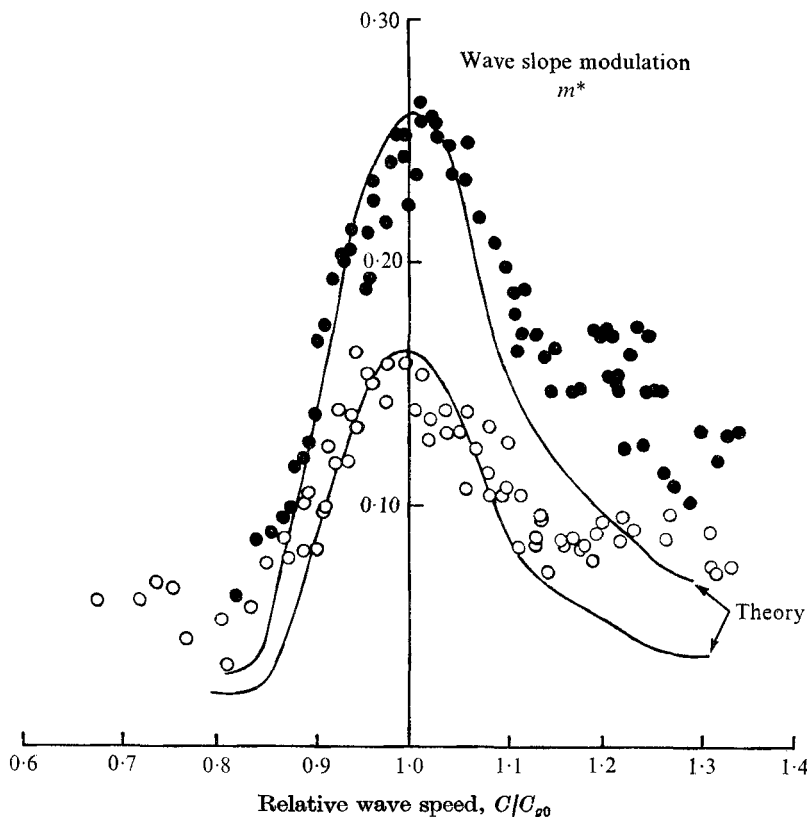
FIGURE 8. Surface-wave slope modulation against relative wave speed, two different interaction configurations with 'matched' values of Kx
