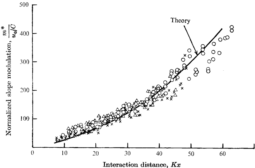
FIGURE 12. Normalized slope modulation against interaction ‘distance’ Kx . C/C_{g0} \simeq 1 .
