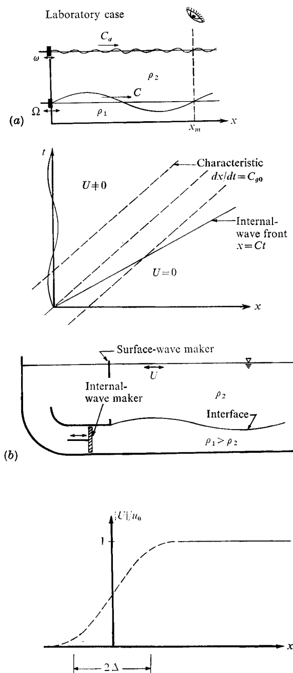
FIGURE 5. (a) Schematic problem definition for laboratory experiment. (b) Schematic diagram of wave tank and estimate of surface current amplitude near wave makers.
