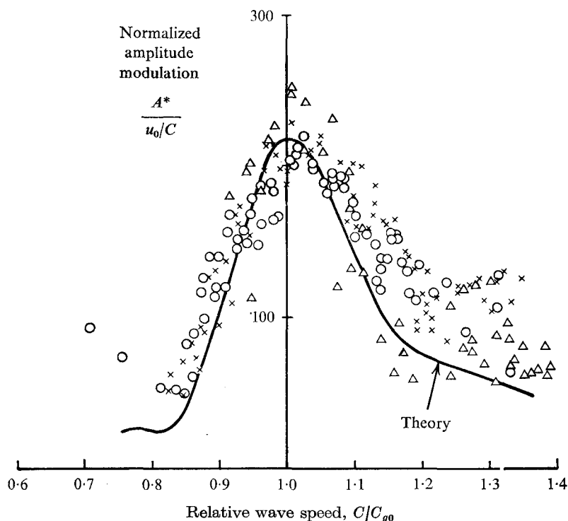
FIGURE 15. Normalized amplitude modulation against relative wave speed. Kx \simeq 43 . Symbols as in figure 14.
