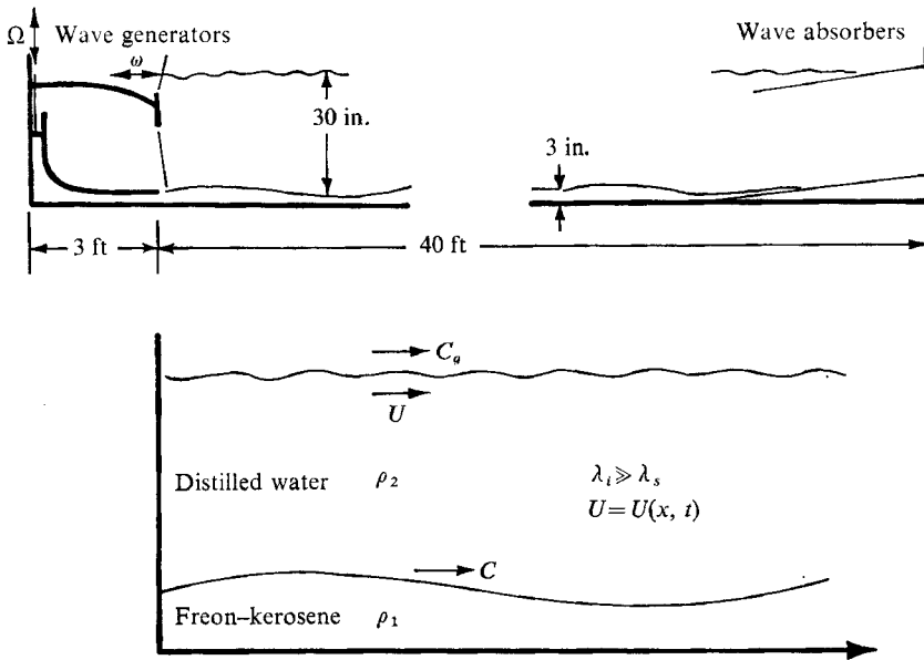
FIGURE 1. Schematic representation of wave interaction experiment.
