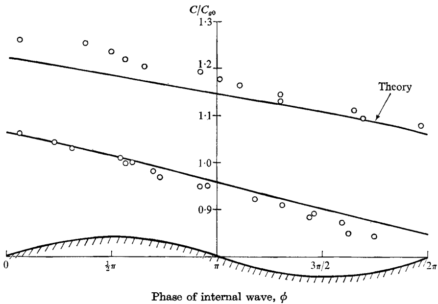
FIGURE 10. Phase location of maximum surface-wave slope modulation for Kx = 42.8 .
