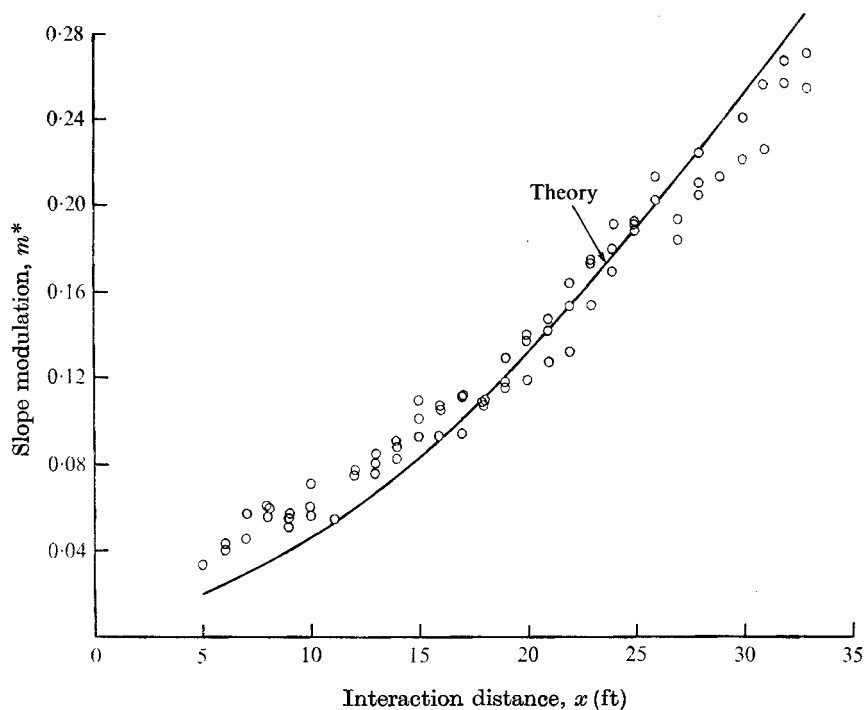
FIGURE 6. Surface-wave slope modulation against interaction distance C/C_{g0} \simeq 1 , \rho = 1.152 , T_i = 3.9 s, k = 1.92 ft ^{-1} , c = 0.84 ft s ^{-1} , \bar{u}_0 = 6.06 \times 10^{-4} ft s ^{-1} .
