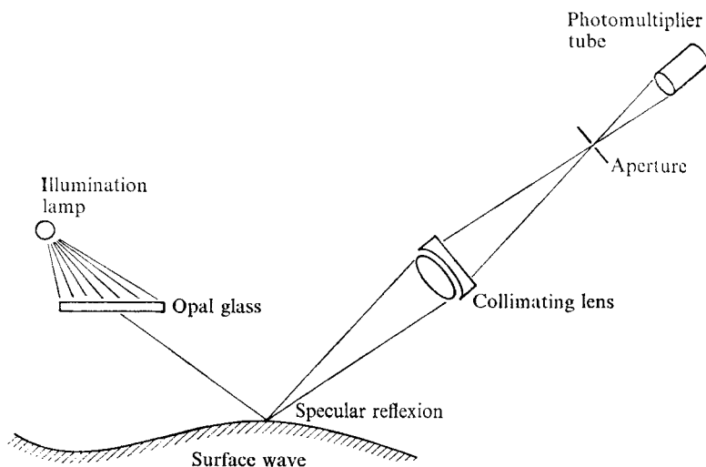
FIGURE 3. Schematic diagram of wave slope measuring device.
