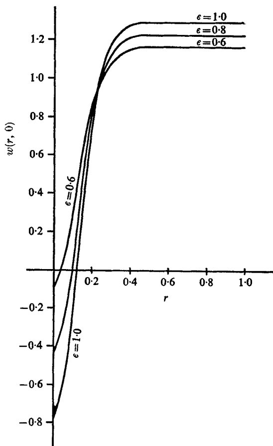
FIGURE 3. The total axial velocity in the breakdown at the plane of symmetry Z = 0 , for various \tilde{\epsilon} , corresponding to figures 1 and 2.
