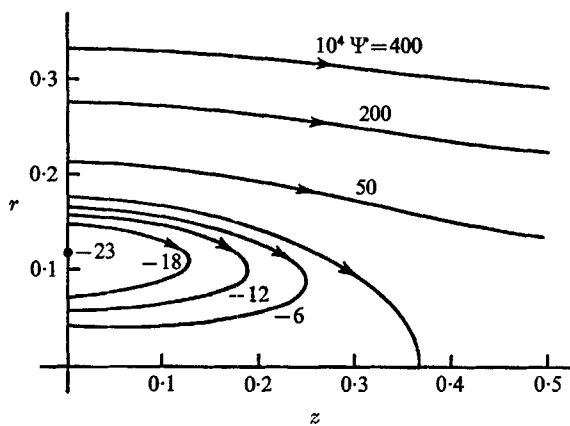
FIGURE 2. Streamlines corresponding to figure 1 in the region of a 'breakdown' eddy, with \tilde{\epsilon} = 1.0 . Unit of length for both axes is the tube radius.
