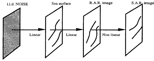
Fig. 1 - 2D SAR imaging process simulation
