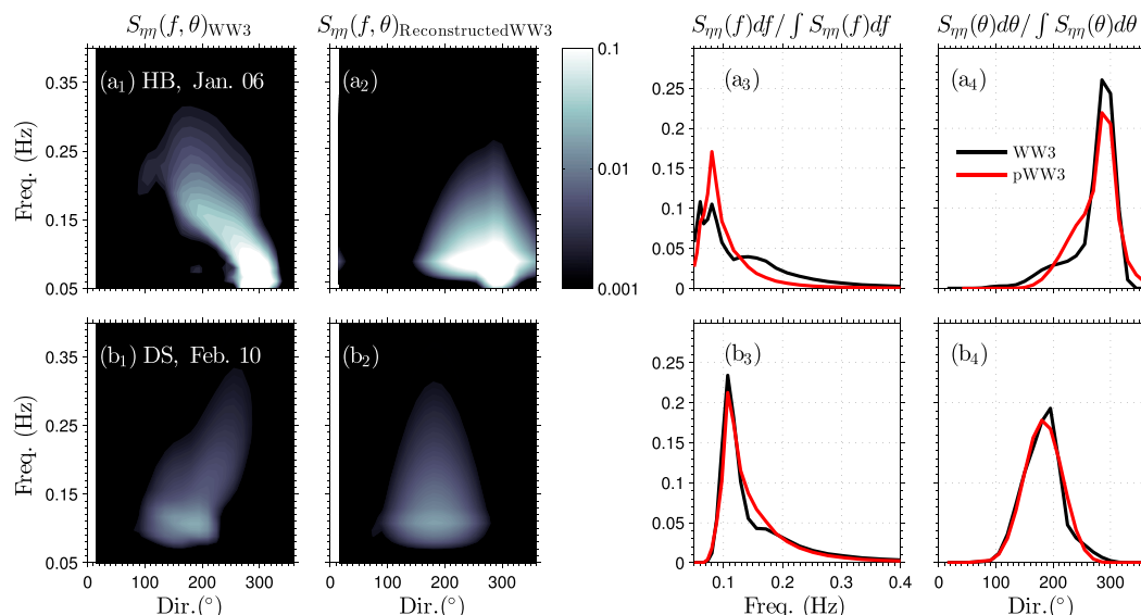
FIG. 3. (a 1 ), (b 1 ) WW3-simulated vs (a 2 ), (b 2 ) reconstructed S_{\eta\eta}(f, \theta) at HB (NDBC ID 46218) in the Southern California Bight at 1200 UTC 2 Jan 2006 in (a 1 ) and (a 2 ) and DS (NDBC ID 41025) in Mid-Atlantic Bight at 0900 UTC 6 Feb 2010 (b 1 ) and (b 2 ). (a 3 ), (b 3 ) Normalized frequency S_{\eta\eta}(f)df / \int S_{\eta\eta}(f)df and (a 4 ), (b 4 ) directional S_{\eta\eta}(\theta)d\theta / \int S_{\eta\eta}(\theta)d\theta spectra from reconstructed (red) and WW3 simulated (black) are also shown.
