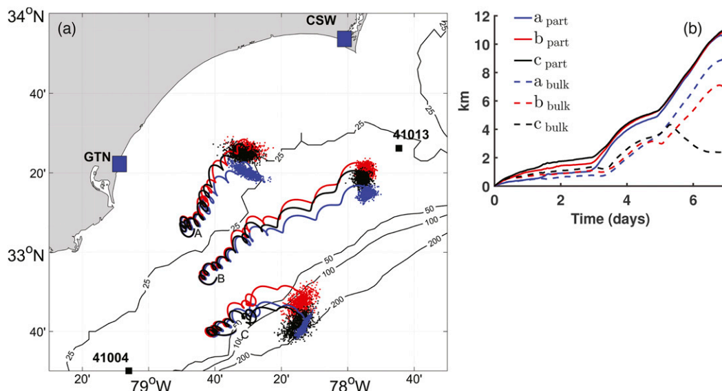
FIG. 9. (a) Lagrangian trajectories estimated over the period of 7 days using HF radar currents u' (blue), Lagrangian-corrected HF radar currents using u_{\text{part}}^L (red), and u_{\text{bulk}}^L (black). Initial locations are labeled as A, B, and C. (b) Separation distance of center of mass (between u_{\text{part}}^L and u' in solid lines, between u_{\text{bulk}}^L and u' in dashed lines) for each trajectory calculation shown in (a) with different starting points (A, B, and C).
