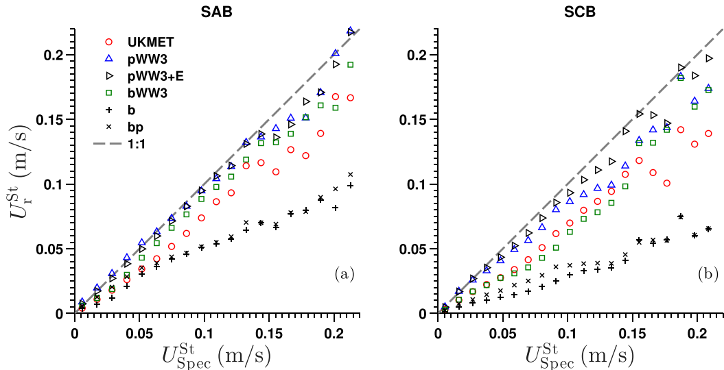
FIG. 11. Bin-averaged surface Stokes drift estimates from reconstructed spectra and bulk parameters U_r^{\text{St}} (see key legend in figure and text for details) vs Stokes drift estimates from WW3 simulated spectra U_{\text{Spec}}^{\text{St}} for (a) the SAB (NDBC buoys 41004 and 41013) and (b) the SCB (NDBC buoys 46218, 46219, and 46222).
