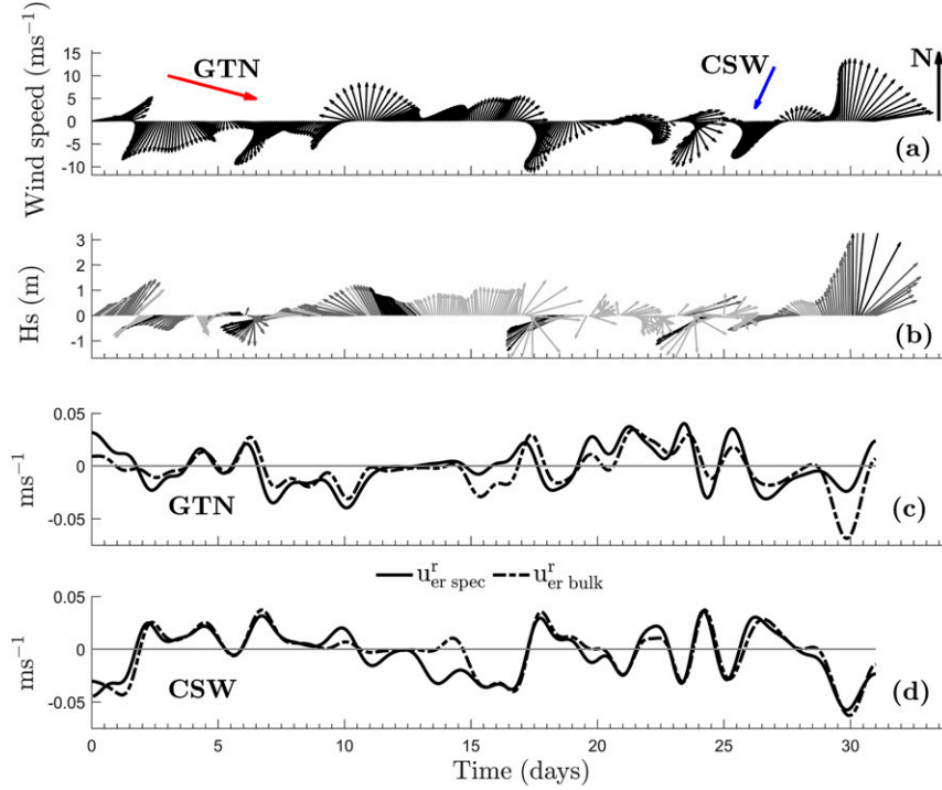
FIG. 8. (a) Time series of low-pass wind velocity vectors; the radial directions from the radar site to the measurement location for each HF radar station (GTN and CSW) are shown as red and blue arrows, respectively. (b) Time series of significant wave height H_s and direction represented as vectors from measurements from NDBC buoy 41013. Color of each vector indicates the number of partitions identified in the spectra (black = 1 partition, gray = 2 partitions, light gray = 3 or more partitions). Comparison of the differences between radial components of surface Stokes and filtered Stokes velocity u_{er}^r [Eq. (9)] estimated using bulk- (dashed) and partition-based spectral reconstruction (solid) for (c) GTN and (d) CSW, respectively.
