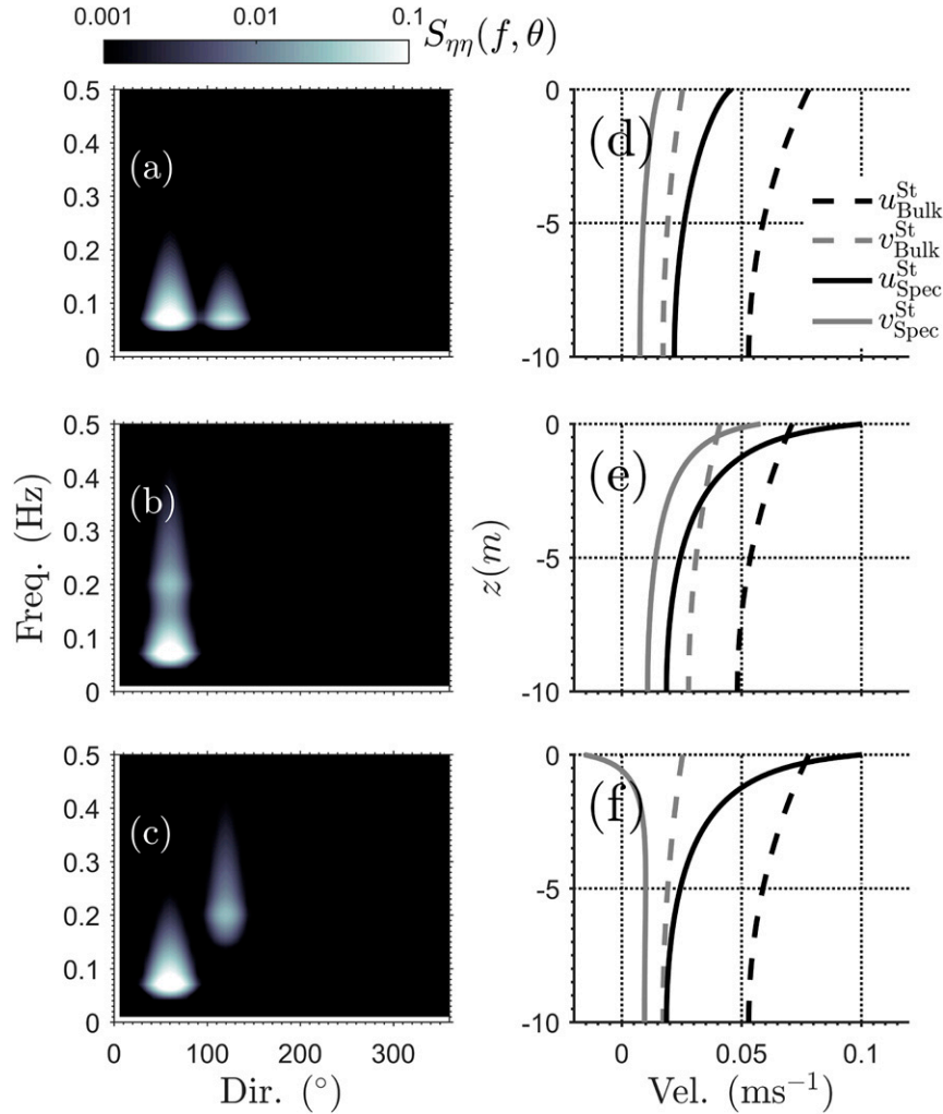
FIG. A1. Directional wave spectra S_{\eta\eta}(f, \theta) ( \text{m}^2 \text{Hz}^{-1} \text{deg}^{-1} ) at h = 10 \text{ m} for three cases corresponding to (a) unimodal, bidirectional; (b) bimodal, unidirectional; and (c) bimodal and bidirectional. North u^{\text{St}} (black) and east v^{\text{St}} (gray) Stokes drift as a function of water depth z estimated using spectral formulation [solid lines; Eq. (A.1a)] and bulk wave parameters [dashed lines; Eq. (A.2)].
