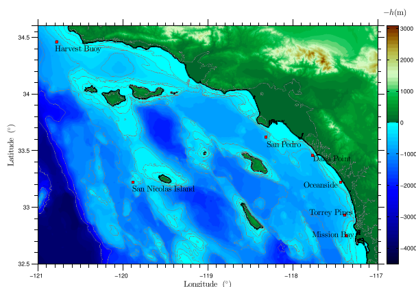
FIG. 4. Model domain used for simulating waves in the Southern California Bight. The color shading represents bathymetry, while red squares show the location of offshore NOAA buoy locations used for model verification and comparison of reconstructed and simulated spectra (see text for details).
