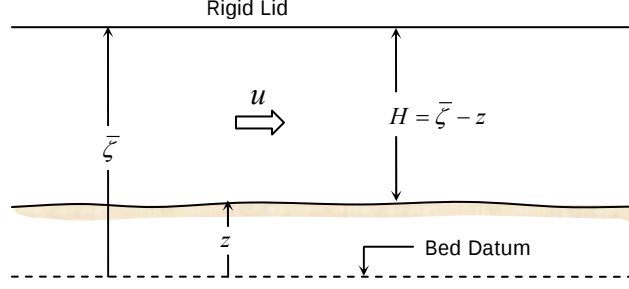
Fig. 1: Definition sketch for Exner's model
