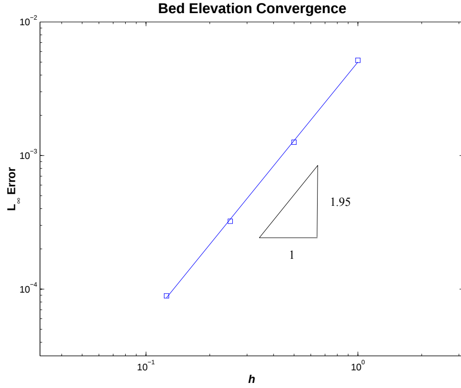
Fig. 6: Convergence plot of test case 1 demonstrating 2 nd order convergence
