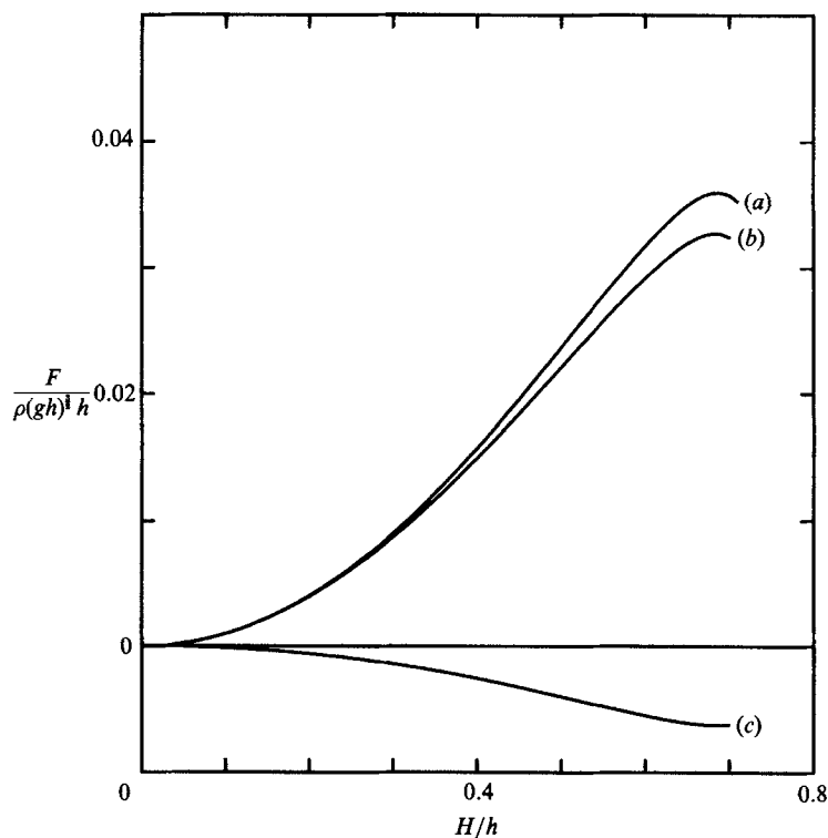
FIGURE 2. Dimensionless mean energy flux F/(\rho(g h)^{1/2} h) as a function of dimensionless wave height H/h for a dimensionless period (\lambda/c)(g/h)^{1/2} = 10 . (a) Stokes's first definition of phase velocity, equation (5.16) of Cokelet (1977) and equation (23); (b) Stokes's second definition of phase velocity, equation (23); (c) Stokes's second definition of phase velocity, equation (5.16) of Cokelet (1977).
