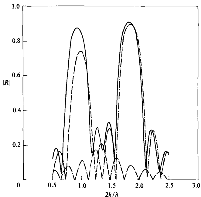
FIGURE 5. Reflection from a patch with two Fourier components, \delta = D_1 \sin \lambda x + D_2 \sin (\frac{15}{8}\lambda x) , n = 4 . ---, D_1/h = 0.32 , D_2/h = 0 ; - · -, D_1/h = 0 , D_2/h = 0.32 ; —, D_1/h = D_2/h = 0.32 .
