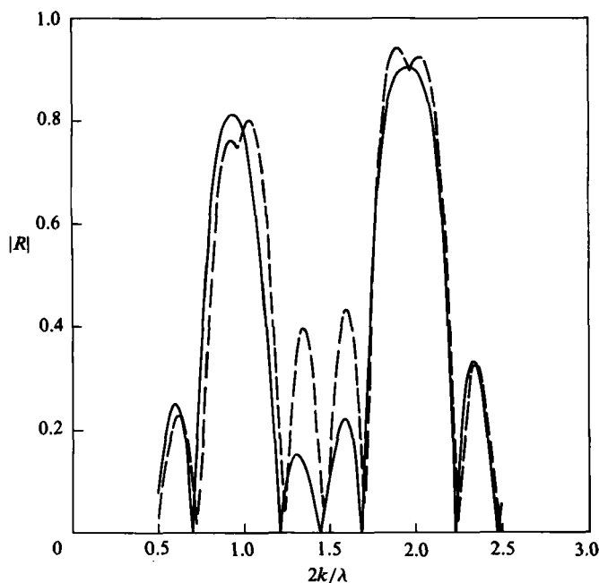
FIGURE 6. Reflection from a patch with two Fourier components \delta = D_1/\sin \lambda x + D_2/\sin 2\lambda x , n = 4 . —, D_1/h = D_2/h = 0.32 (as in figure 5). ---, sum of individual results for D_1/h = 0.32 , D_2/h = 0 and D_1/h = 0 , D_2/h = 0.32 .
