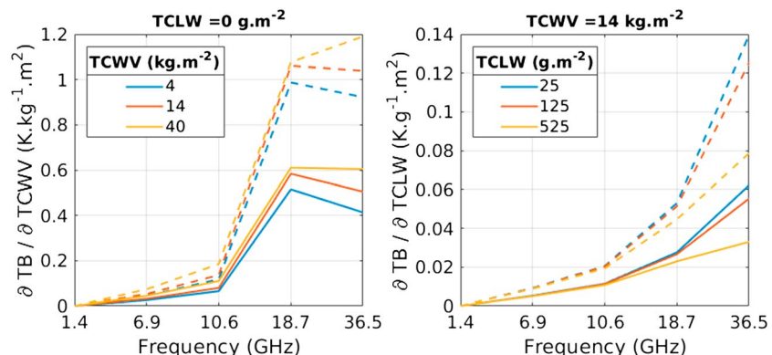
Figure 4. The TCWV (left) and the TCLW (right) Jacobians at Copernicus Imaging Microwave Radiometer channels and at an incidence angle of 55^\circ for different TCWVs and TCLWs (colors), respectively. Vertical and horizontal polarizations are, respectively, plotted as solid lines and dashed lines. The sea surface temperature is set at 285 K, the ocean wind speed is set at 6 m/s, and the sea surface salinity is set at 36 psu. TCWV = Total Column Water Vapor; TCLW = Total Column Liquid Water; TB = brightness temperature.
