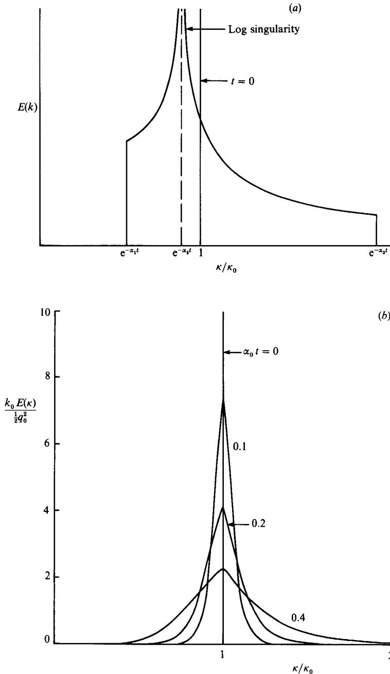
FIGURE 8. The change in a delta-function spectrum of small-scale turbulence undergoing random irrotational straining by large-scale turbulence. (Rotational straining does not affect \bar{E}(\kappa) over short times.) (a) The fixed magnitudes of principal strains, but random orientations, \alpha_1 > \alpha_2 > \alpha_3 , where \alpha_2 > 0 ; (b) Gaussian distribution of strains with variance \alpha_0^2 .
