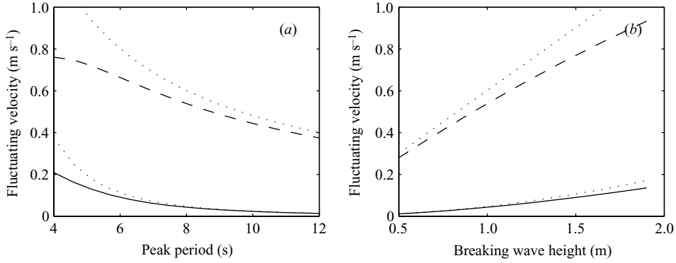
FIGURE 2. Maximum longshore (—) and cross-shore (—) velocities from (3.7)–(3.8); and asymptotic limits (···) (3.11) from unsteady multidirectional wave forcing using a simplified two-component model with circulation calculated from (3.16)–(3.17). Base case: T_p = 8 s, m = 0.03 , \Delta k = 0.2\kappa_0 , \theta_0 = 0 , \Delta f = 0.2f_p , H_b = 1 m, \gamma = 0.78 . (a) Changing peak period; (b) changing breaking wave height.
