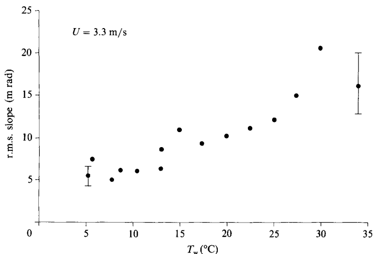
FIGURE 11. Root-mean-square slope at fixed ( U = 3.3 m/s) wind speed vs. water temperature. The bars refer to the \pm 20\% accuracy of the visual measurement (cf. figure 2).
