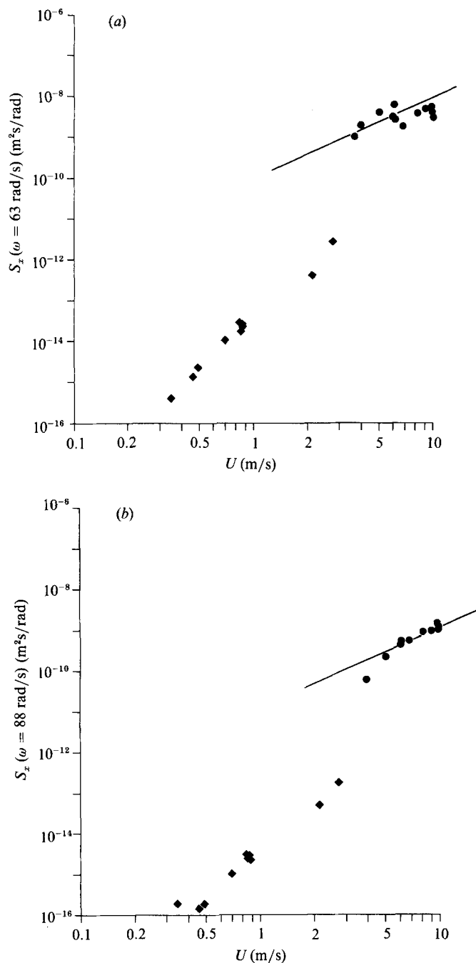
FIGURE 8. Growth with wind speed of single components on the rear face of the wave spectrum. \bullet , capacitance gauge; \blacklozenge , transformed from slope gauge. The line has a slope of 2.
