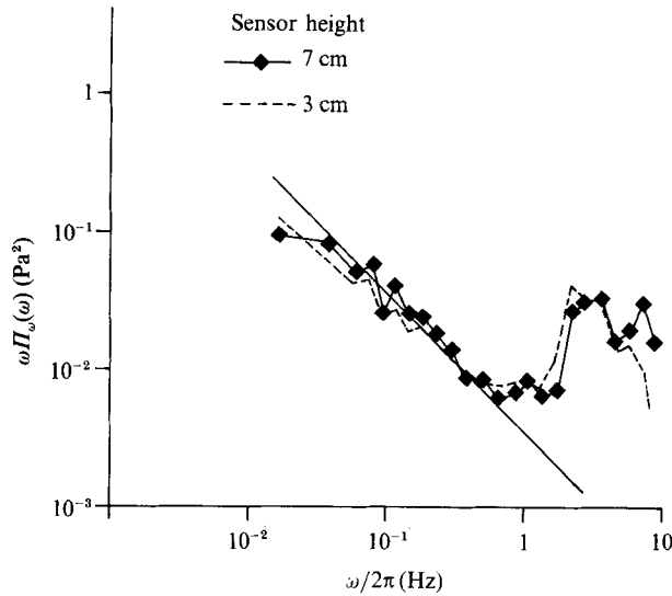
FIGURE 12. Frequency spectra of pressure fluctuations over water in a large wind wave flume ( x = 55 m, water depth 1.2 m, height of the air flow 1.86 m) at u_* = 18 cm/s. The line shows the extrapolation into high frequencies where the measured spectra show wave-induced fluctuations and noise.
