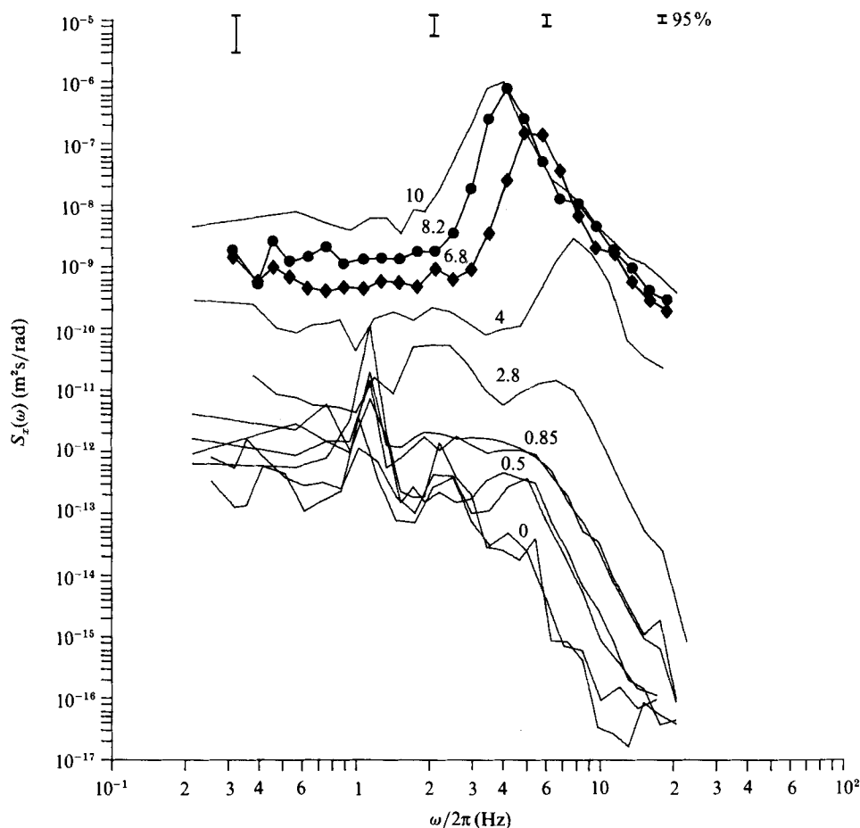
FIGURE 4. The evolution of the frequency spectrum with wind speed (indicated on the figure). The spectra at 0, 0.5, 0.85 and 2.8 m/s wind speed are composites derived from surface displacement spectra and transformed slope spectra.
