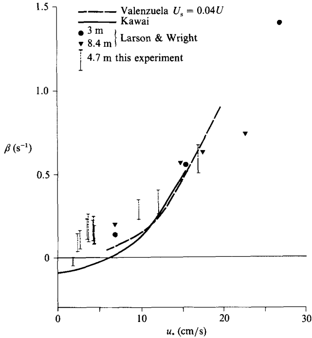
FIGURE 6. Exponential growth rate \beta for waves in the x -direction ( T_w = 25^\circ\text{C} ). For our observations the most probable value for \beta is close to the minimum of the bar.
