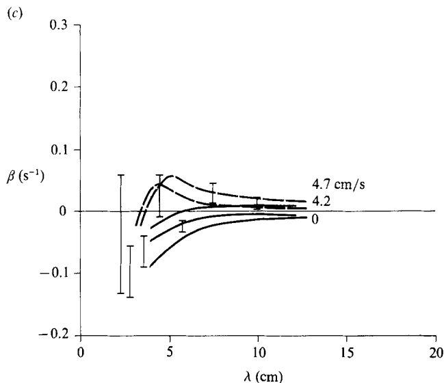
FIGURE 5. Exponential growth rate \beta for waves in the x -direction ( T_w = 25^\circ\text{C} ). The bar length refers to the maximum variability which is consistent with (6). The most probable value for \beta is expected to be close to the minimum of the bar. The curves are from the instability theory (Kawai 1979b). (a) u_* = 3.4 cm/s, U = 0.7 m/s; (b) u_* = 2.8 cm/s, U = 0.48 m/s; (c) u_* = 1.9 cm/s, U = 0.35 m/s.
