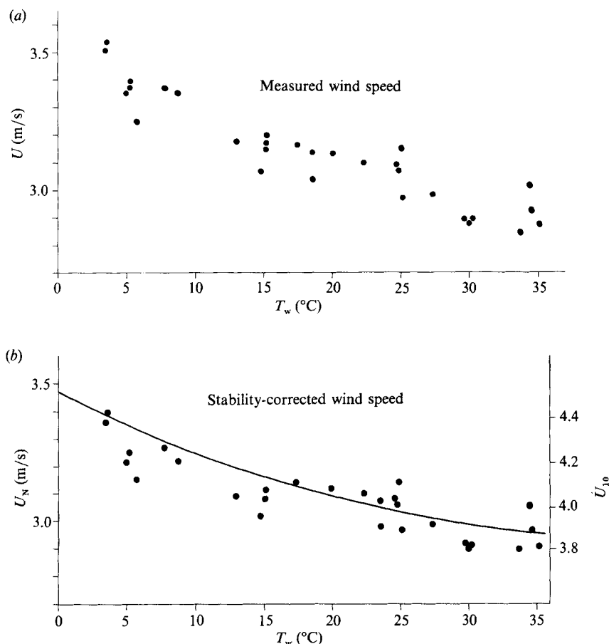
FIGURE 10. Critical wind speed at 0.156 m height vs. temperature. The 6.6 mrad r.m.s. slope at the critical wind speed was determined by the visual method. The line (figure 10b) shows the predicted temperature dependence based on our observed \beta at fixed 25 °C temperature (figure 6) and assuming \beta_d = -4 k^2 \nu_w .
