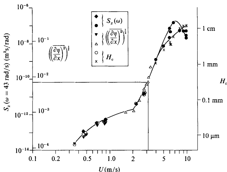
FIGURE 7. Growth vs. wind speed of a single component of the displacement spectrum near the peak ( \blacklozenge , \bullet ); r.m.s. slope ( \blacktriangledown , \triangle ); and characteristic wave height ( \circ , \times ). The measurement methods used were: \blacklozenge , \blacktriangledown , \circ , slope gauge; \bullet , \times , capacitance gauge; \triangle , visual method. The vertical line shows the critical wind speed which corresponds to 6.6 mrad r.m.s. slope. The water temperature was 25 °C.
