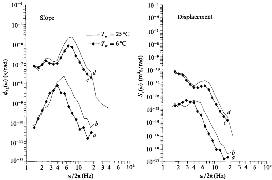
FIGURE 9. Displacement and slope spectra at two temperatures. (a) T_w = 6^\circ\text{C} , U = 0.76 m/s; (b) T_w = 25^\circ\text{C} , U = 0.48 m/s; (c) T_w = 6^\circ\text{C} , U = 2.9 m/s, U_N = 2.7 m/s; (d) T_w = 25^\circ\text{C} , U = U_N = 2.8 m/s.
