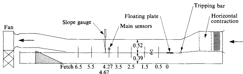
FIGURE 1. The wind-wave flume.
