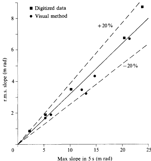
FIGURE 2. Calibration of the visual method to determine the r.m.s. slope.
