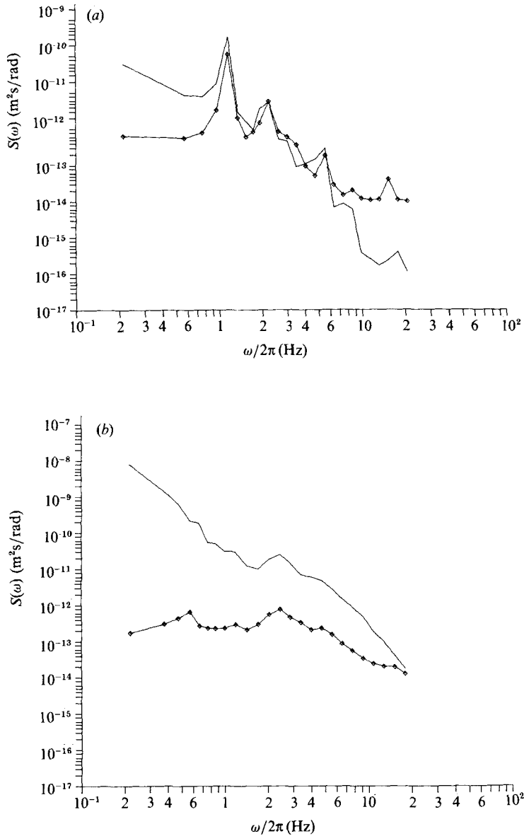
FIGURE 3. Comparison between the displacement spectrum from a capacitance gauge ( -\diamond- ) and the transformed slope spectrum ( --- ). (a) example of agreement found in 50% of the cases; (b) the worst case observed.
