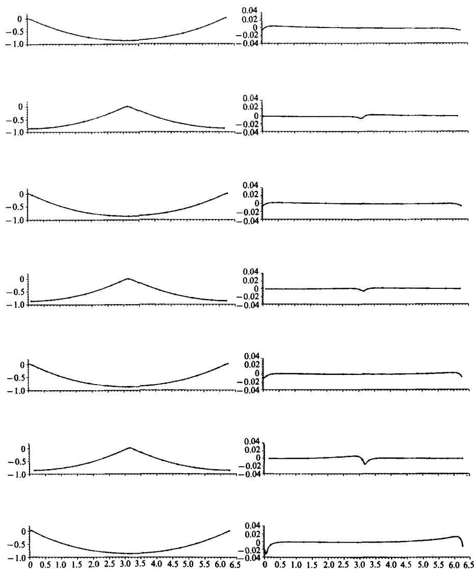
FIGURE 7. The time development of the rapidly decaying \omega = 0.82 wave unstable mode started with \varepsilon = -0.01 laid out as in figure 4. The time development is taken from t = 0 to t = 17.25 with plots made every half-wave period ( t = 2.875 ) downwards.
