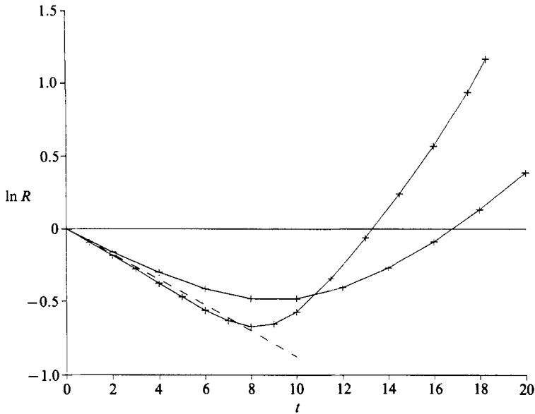
FIGURE 6. Decay and growth of the \omega = 0.82 wave decaying modes with perturbation magnitude |\epsilon| = 0.01 plotting \ln R against time. The predicted linear decay is shown by the dashed line. The slowly decaying solution has \epsilon = 0.01 and the rapid decay has \epsilon = -0.01 .
