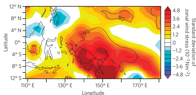
Figure 4 | Intraseasonal zonal wind stress variations in the western Pacific in December–March after a negative IOD. Standard deviation of 30–100 days' band-pass-filtered zonal wind stress in DJFM partially regressed to minus the IOD index, with the ENSO influence removed ( 10^{-3}\text{ N m}^{-2} , 90% significance level in black contours).
