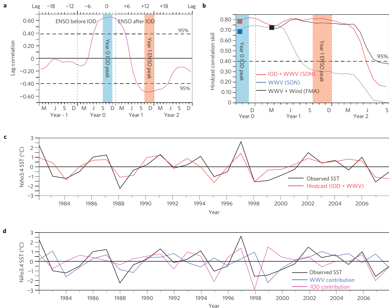
Figure 1 | IOD index as a precursor of the following year's ENSO state. a, Lag-correlation between IOD (in September–November of year 0) and ENSO indices (dashed lines indicate the 95% confidence limit). b, Correlation skill of Niño3.4 SST hindcasts using WWV and western Pacific zonal wind in February–April of year 1 (black), using only WWV in September–November of year 0 (blue), or WWV + IOD index in September–November of year 0 (red). c, Observed (black) and predicted (red) ENSO index using the WWV and IOD indices of September–November 13 months before. d, Black curve as in c ; the hindcast in c (red) is the sum of the WWV (blue) and DMI (purple) contributions shown in d .
