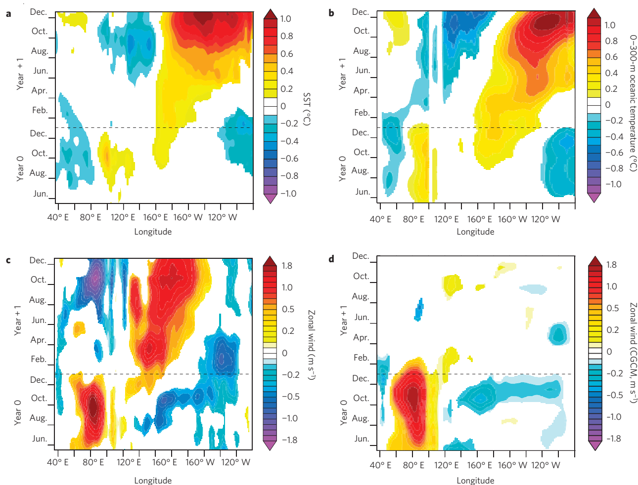
Figure 2 | Longitude-time section of Indo-Pacific anomalies associated with a negative IOD. a , Observed SST (°C). b , 0–300-m oceanic temperature (°C). c , Zonal wind ( \text{m s}^{-1} ) over the Indo-Pacific during and after a negative IOD event (the influence of ENSO has been removed, see the Methods section). d , Indo-Pacific zonal wind signals associated with the IOD in a coupled model experiment with no coupling over the tropical Pacific. Signals are within 2^{\circ}\text{S} – 2^{\circ}\text{N} , except for SST (within 5^{\circ}\text{S} – 5^{\circ}\text{N} in the Pacific, and 10^{\circ}\text{S} – 0^{\circ}\text{N} to the west of 120^{\circ}\text{E} ). Only signals significant at the 90% level are plotted. The dashed line marks the transition from year 0 to year 1.
