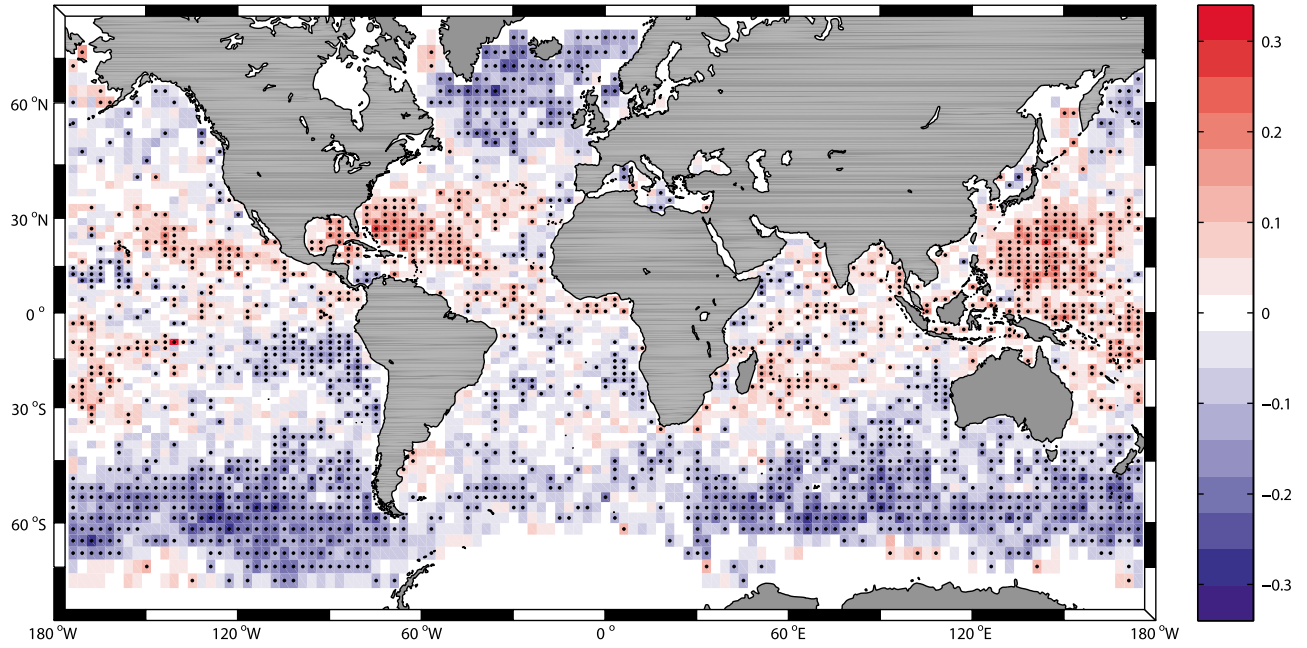
Figure 1. Spatial variability of the shape parameter of extreme wave height distribution around the world. Only statistically significant values at the 90% confidence interval are dotted.
