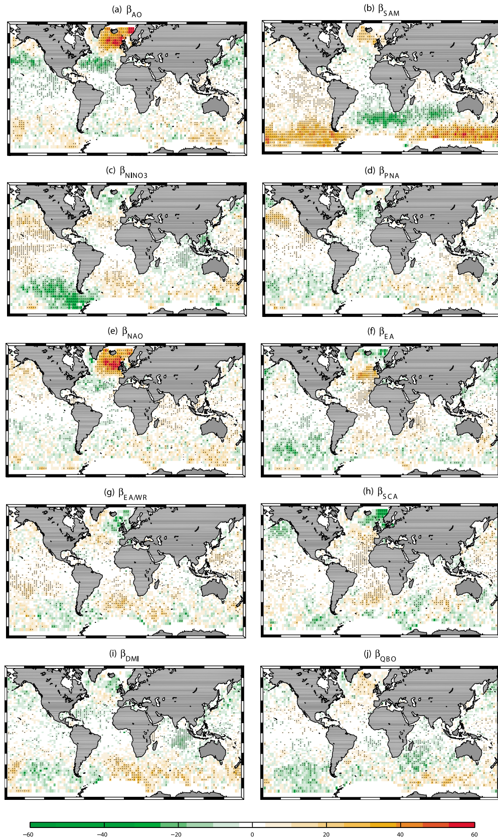
Figure 3. Spatial variability of the influence of the climate indices on the location parameter (cm/unit). Only statistically significant values at the 90% confidence interval are dotted. All figures are bounded to -60 and 60 cm.
