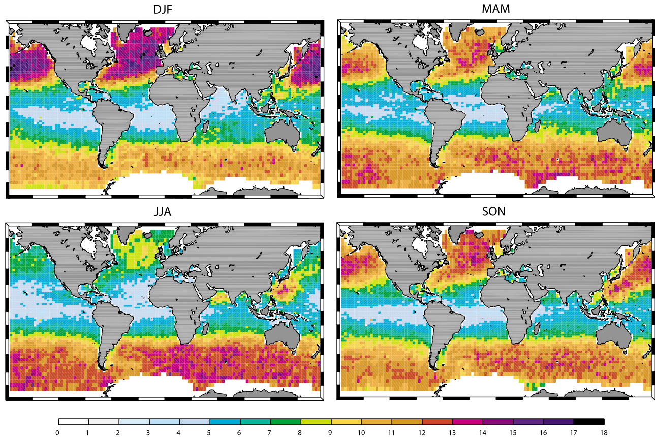
Figure 2. Seasonal distribution of the 20-year return level quantile, H_{s_{20}} (m).
